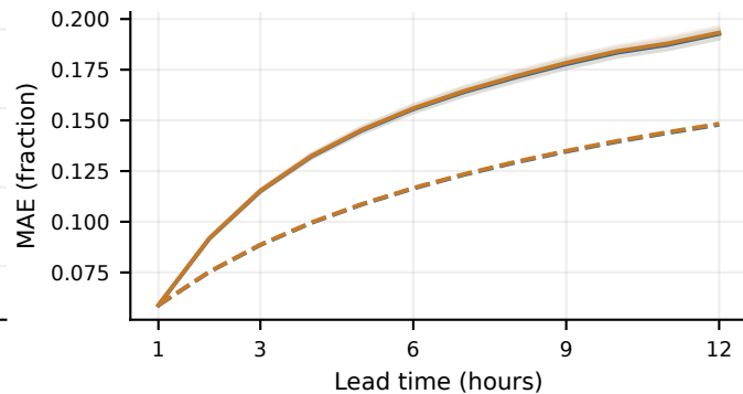
Cloud cover
