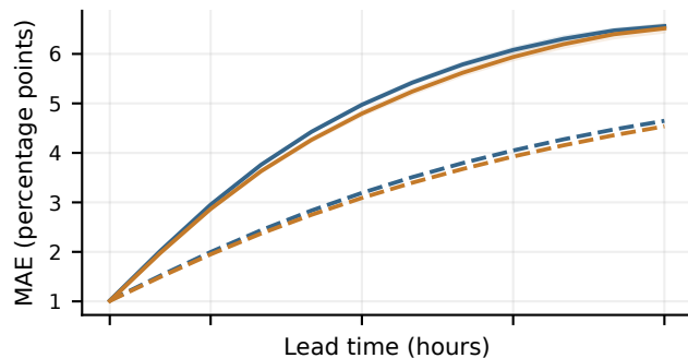
Cloud cover
