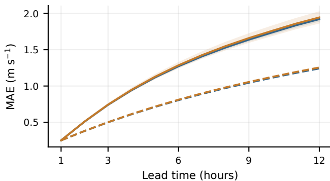
Surface wind
