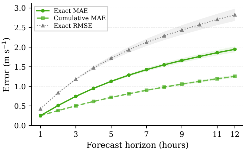
Wind
