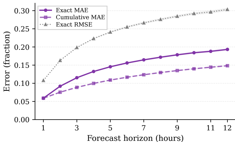
Cloud Cover
