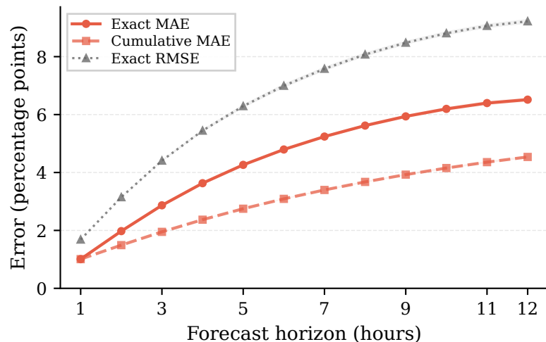
Cloud Cover
