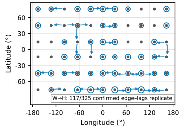
(c) Replicated wind→humidity edges
