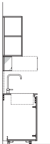
With sink on base D 595 mm. The open modules can be reduced in height to a minimum of 150 mm
