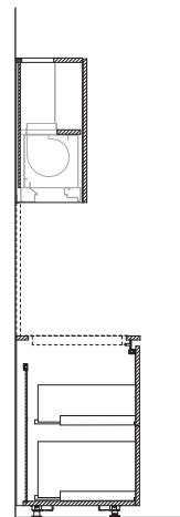
Modula storage units cannot be used with hob on base D 595 mm
