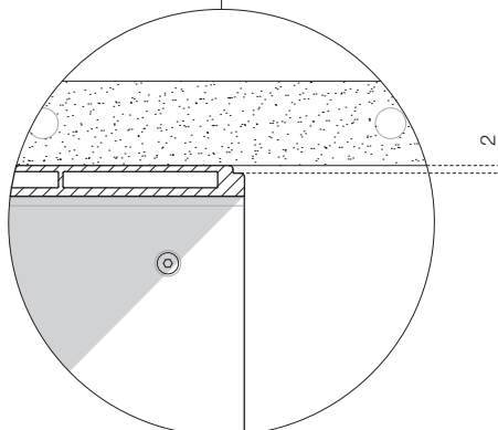
With sink on base D 595 mm. The open modules can be reduced in height to a minimum of 150 mm
