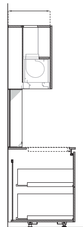
With hob on base D 745 mm use the module without shelves, with Scotch Brite stainless steel back panel and increase the depth of the side panels on the units to a depth of 472 mm.
