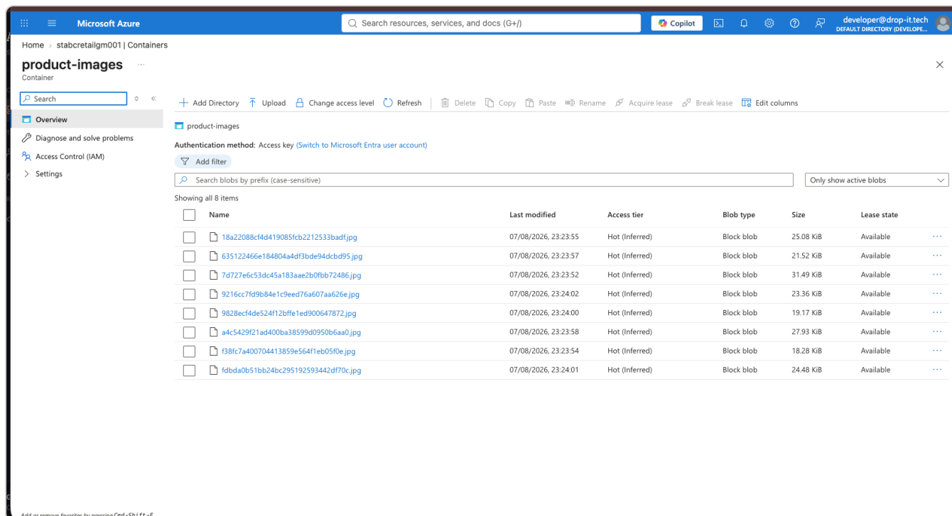
Figure 10. Azure screenshot.
