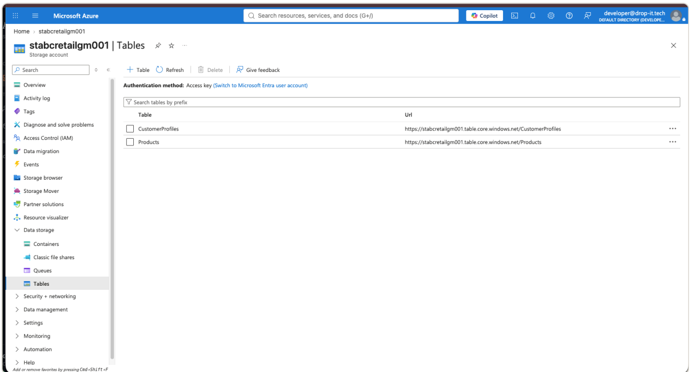
Figure 9. Azure screenshot.
