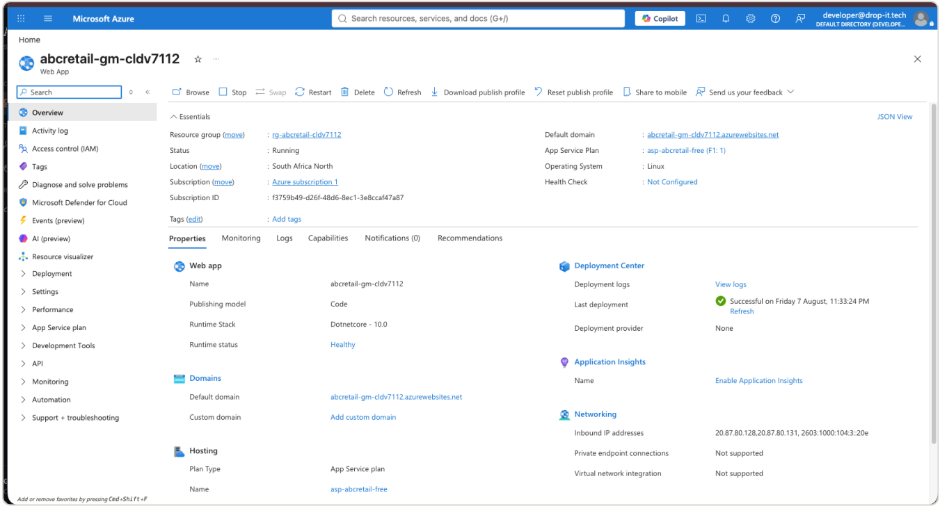
Figure 8. Azure screenshot.
