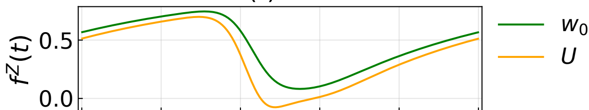
STP factors f^Z(t)
