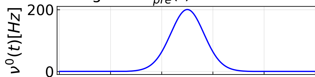
Firing rate v_{pre}^0(t)
