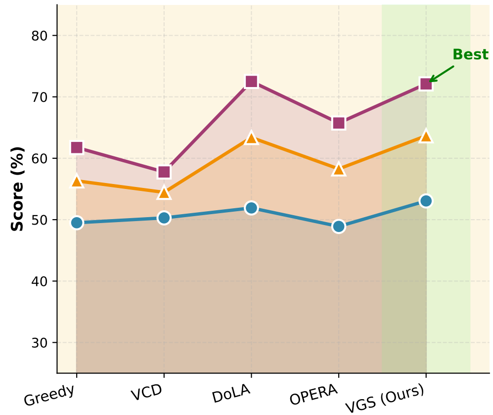
(c) MedGemma
