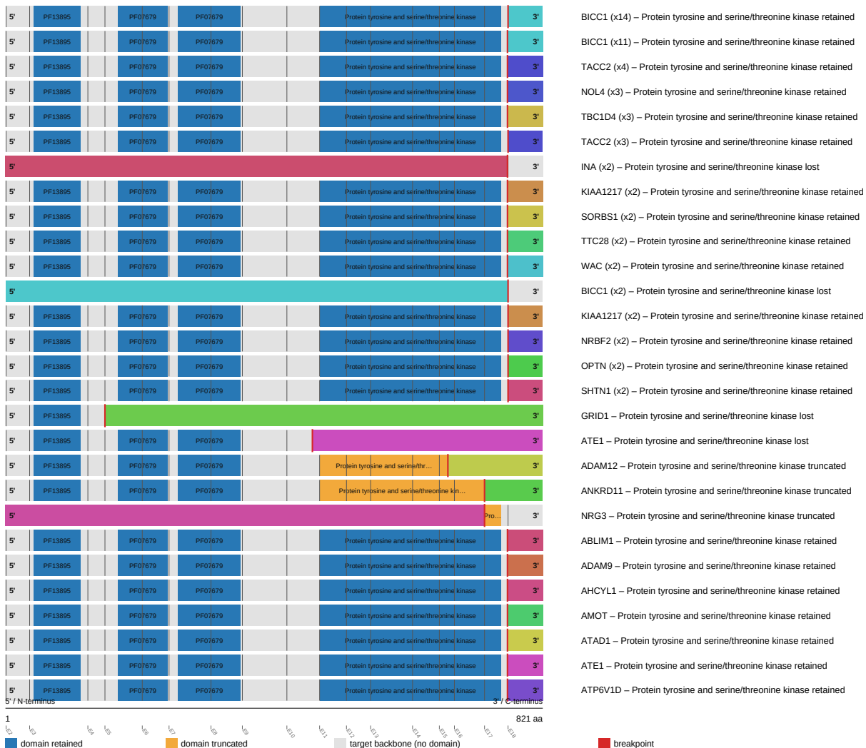
FGFR2 fusion-transcript schematic
