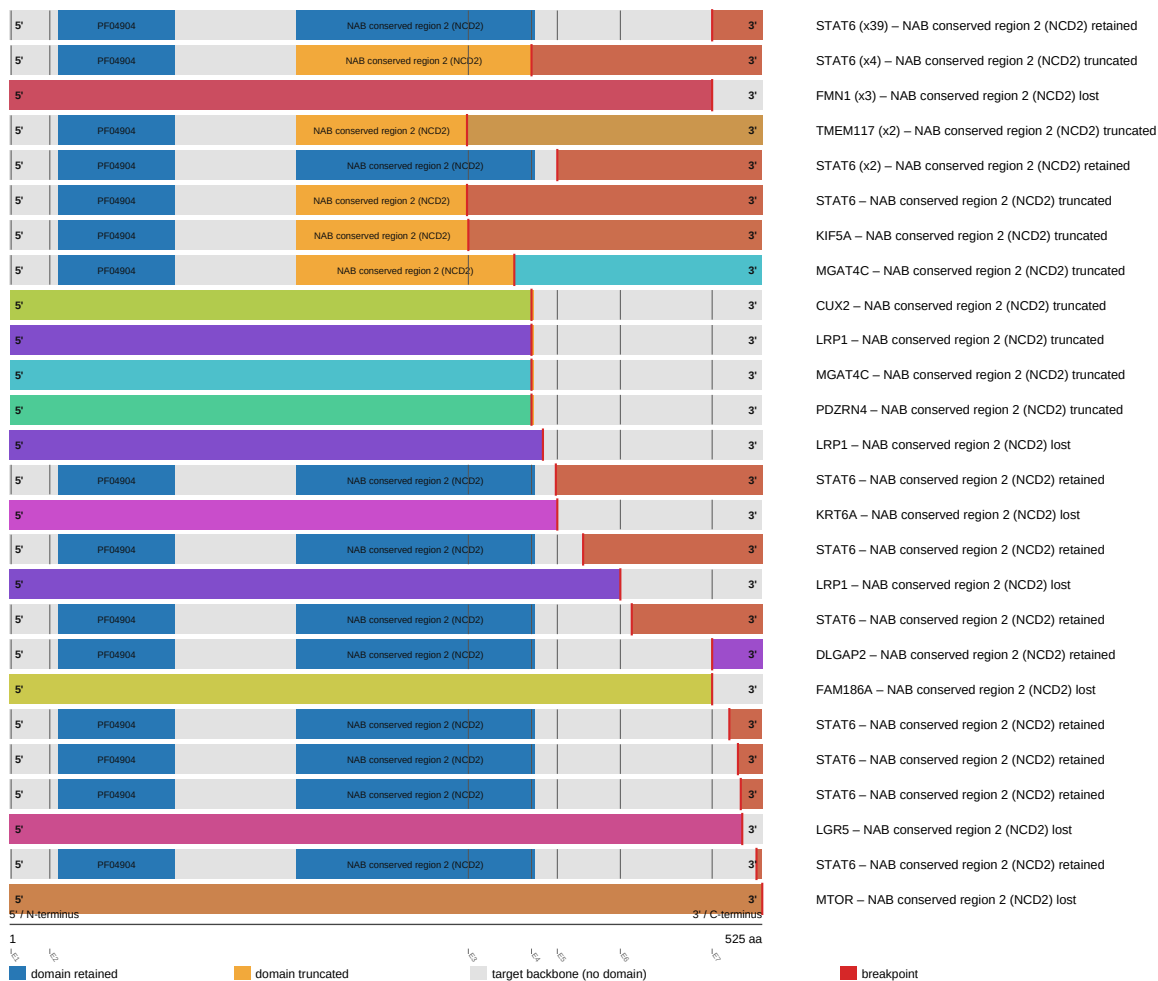
NAB2 fusion-transcript schematic
