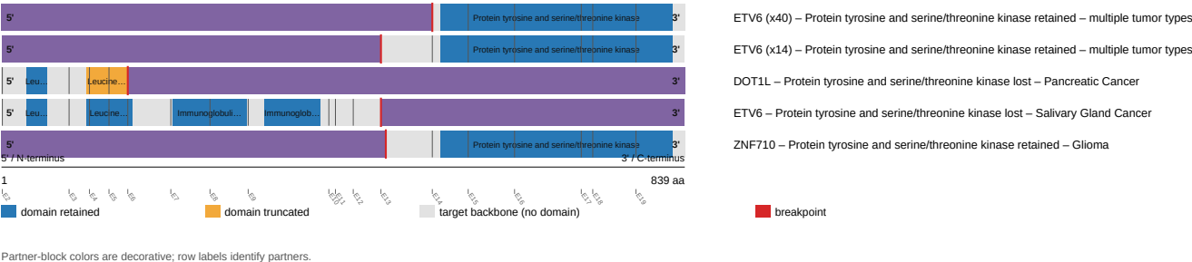
NTRK3 fusion-transcript schematic
