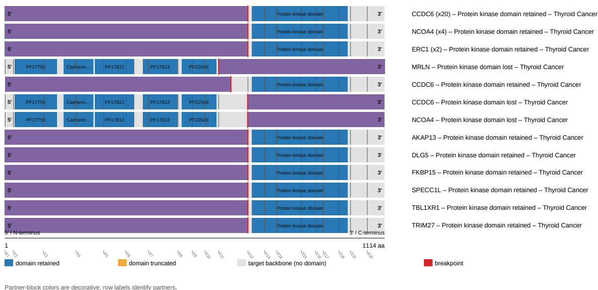
RET fusion-transcript schematic
