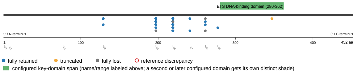
FLI1 domain-retention track
