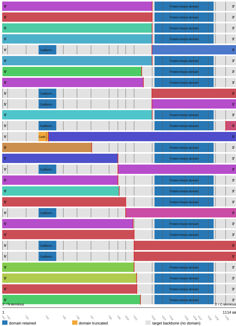
RET fusion-transcript schematic
