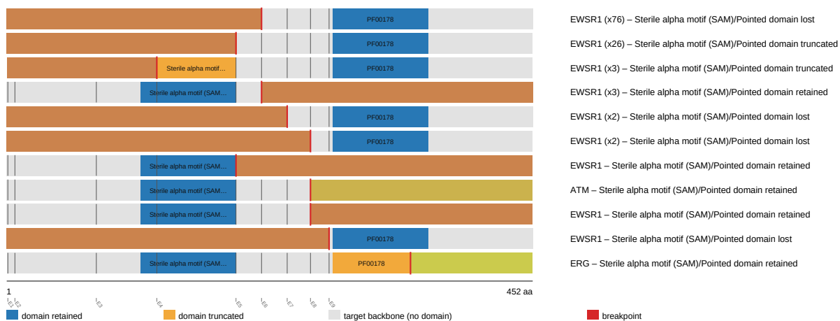
FLI1 fusion-transcript schematic
