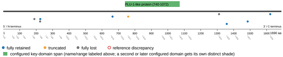
KDM5A domain-retention track
