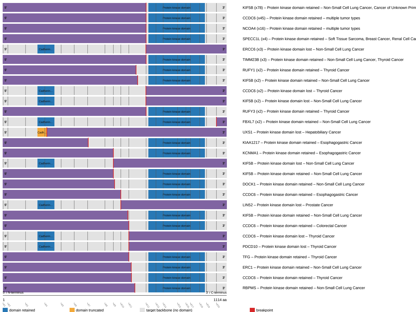
RET fusion-transcript schematic
