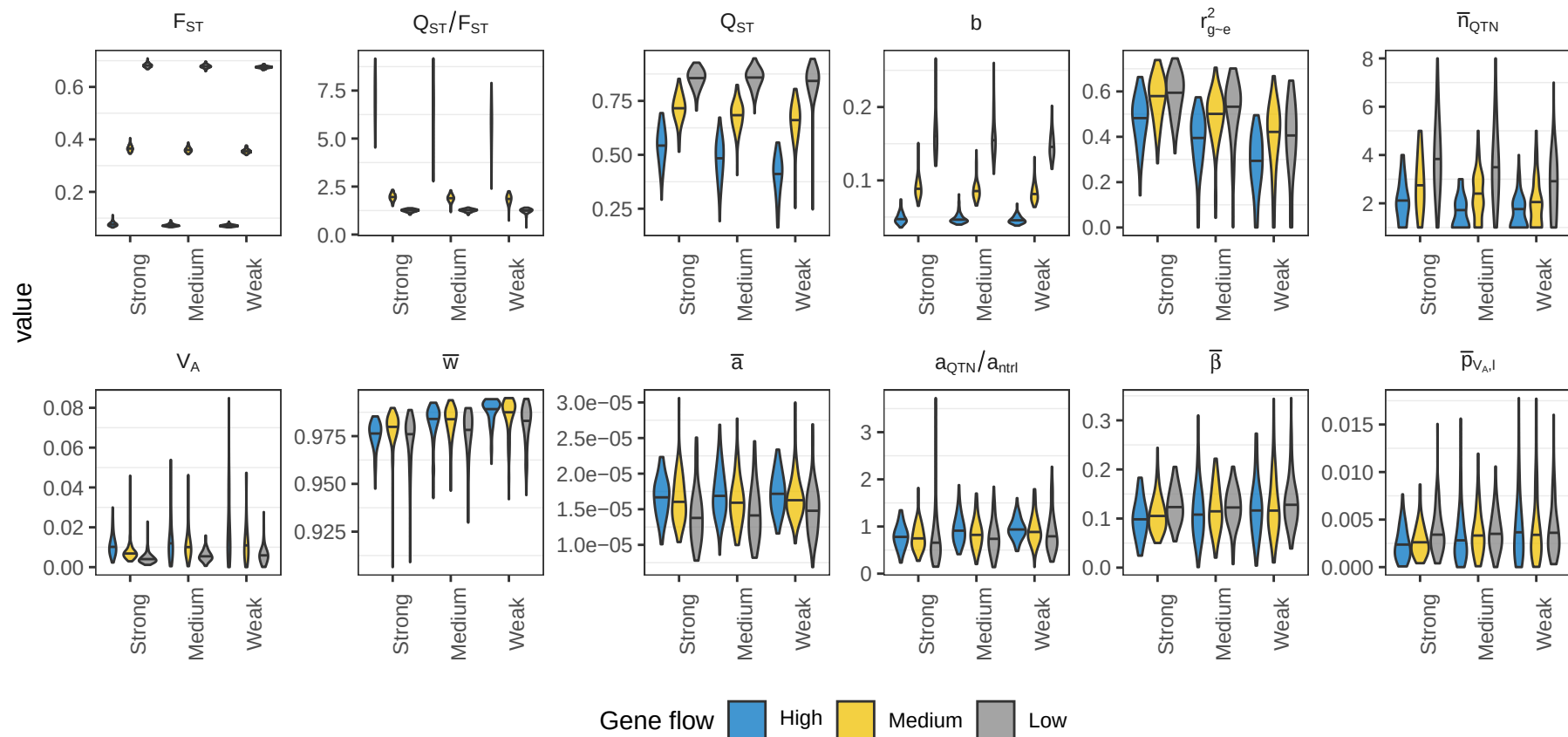
a) Effects of simulation parameters on population demography and local adaptation
