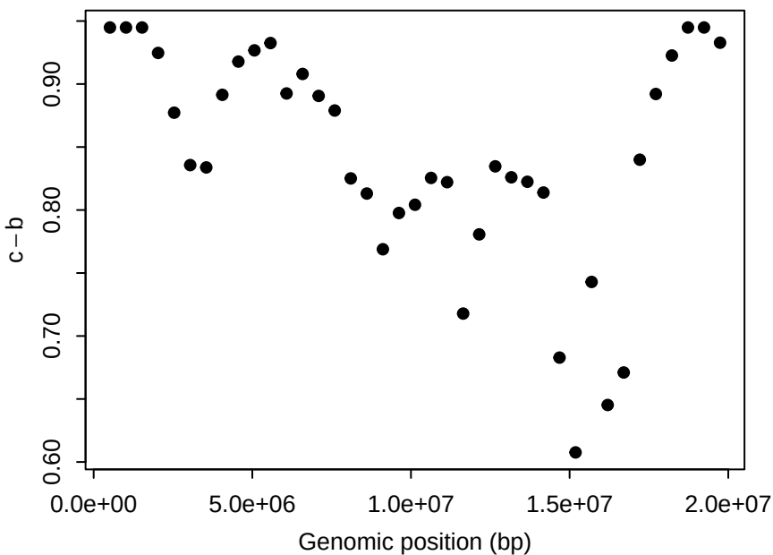
Chr9: LD contrast across windows
