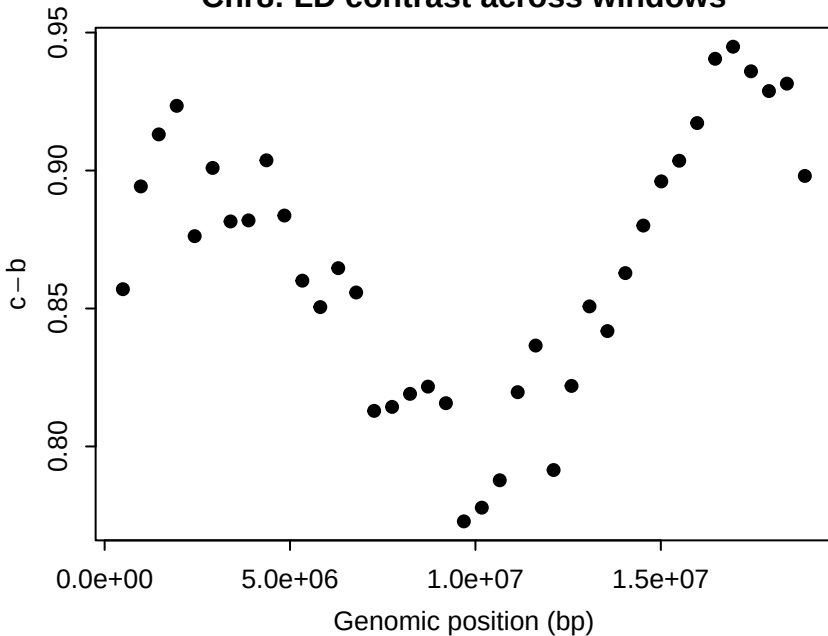
Chr8: LD contrast across windows
