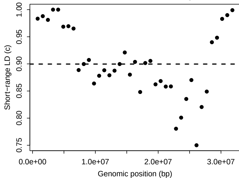
Chr4: fitted decay curves
