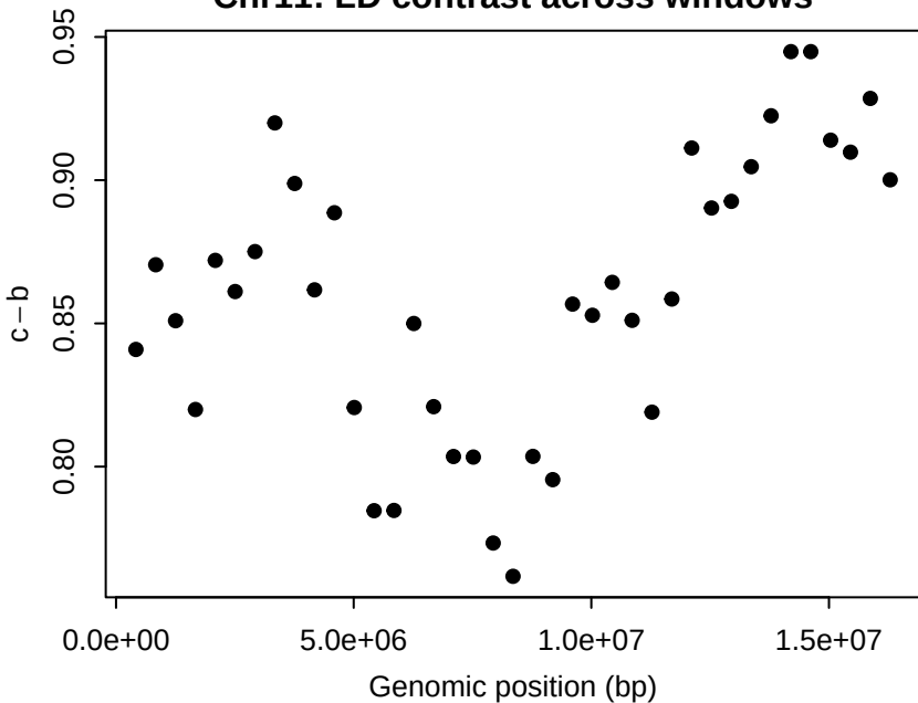
Chr11: LD contrast across windows
