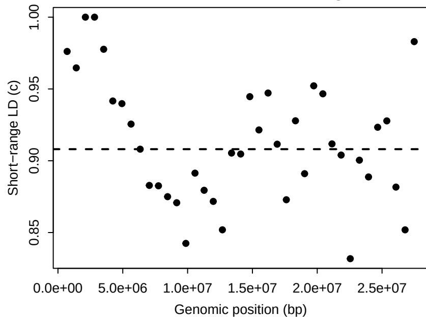
Chr1: fitted decay curves
