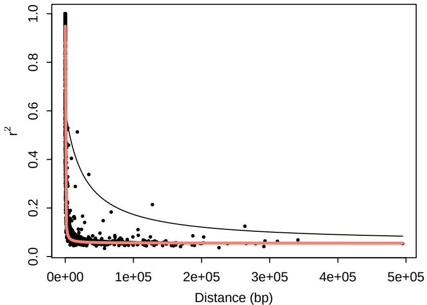
Chr17: fitted decay curves
