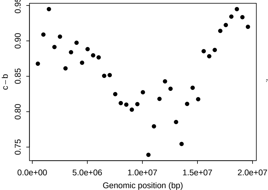
Chr13: LD contrast across windows
