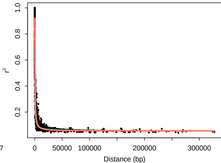
Chr13: fitted decay curves
