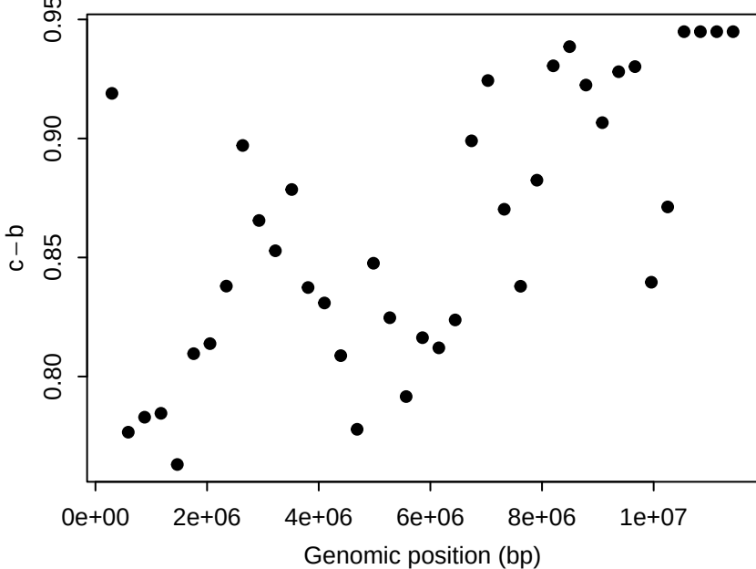
Chr21: LD contrast across windows
