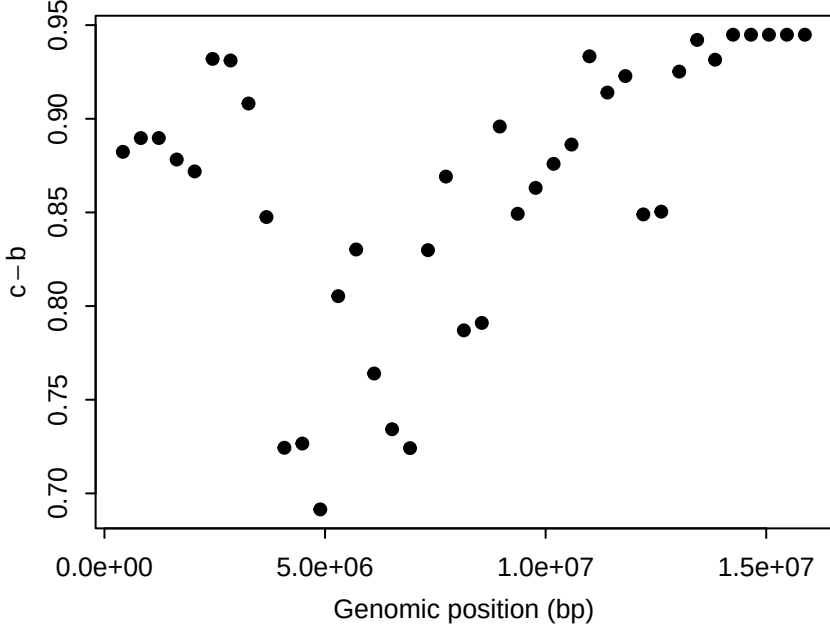
Chr18: LD contrast across windows
