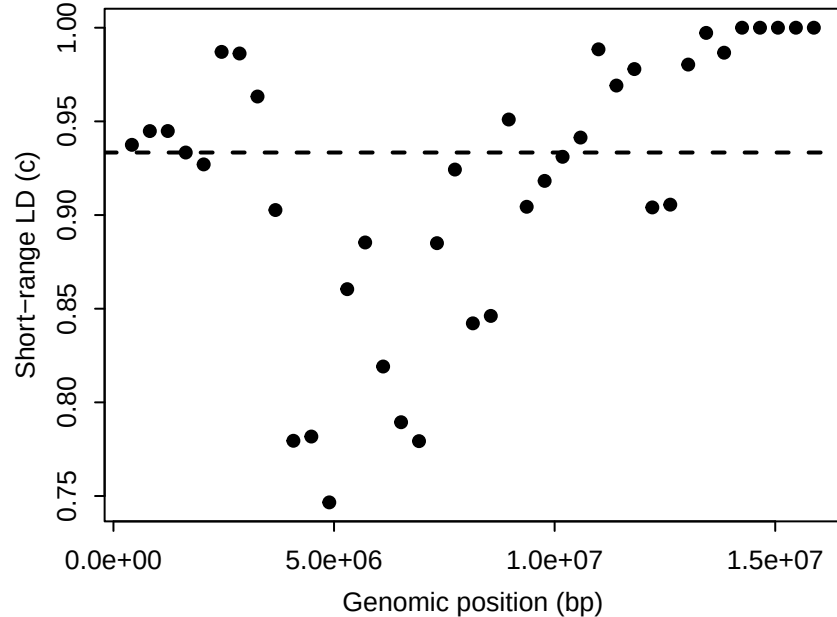
Chr18: fitted decay curves
