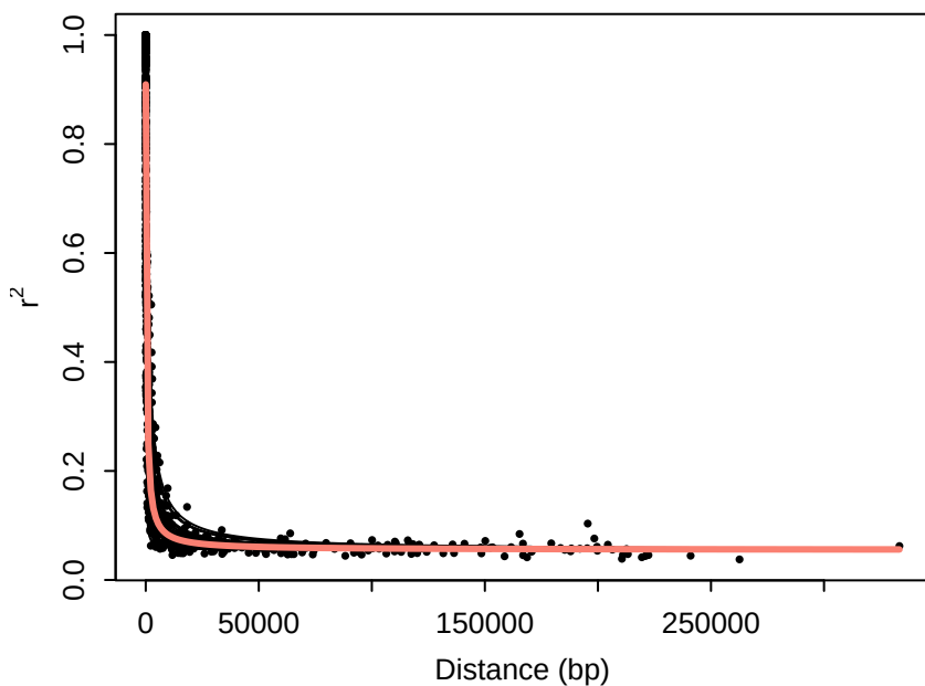
Chr15: fitted decay curves
