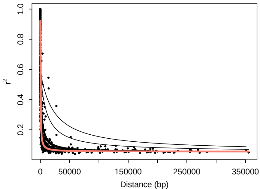
Chr5: fitted decay curves
