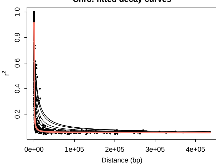
Chr8: fitted decay curves
