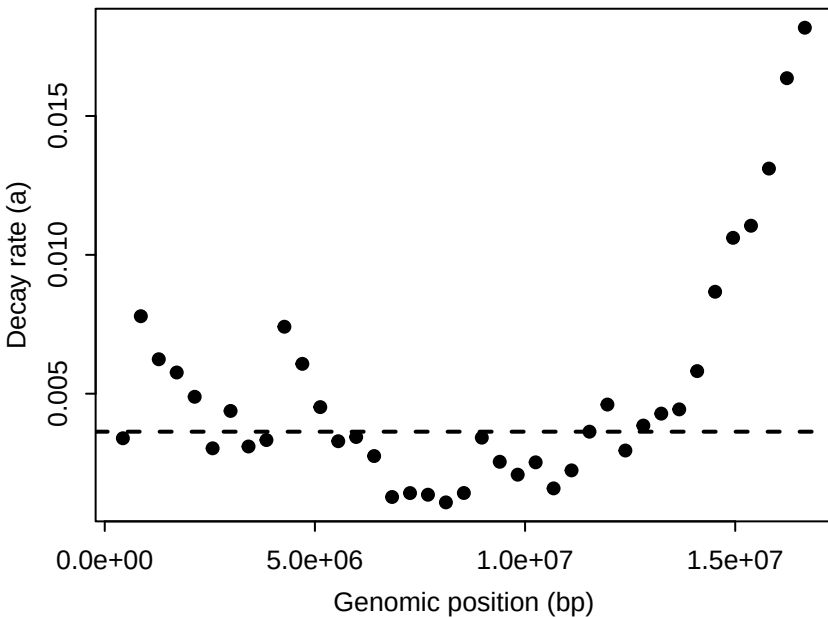
Chr6: LD contrast across windows
