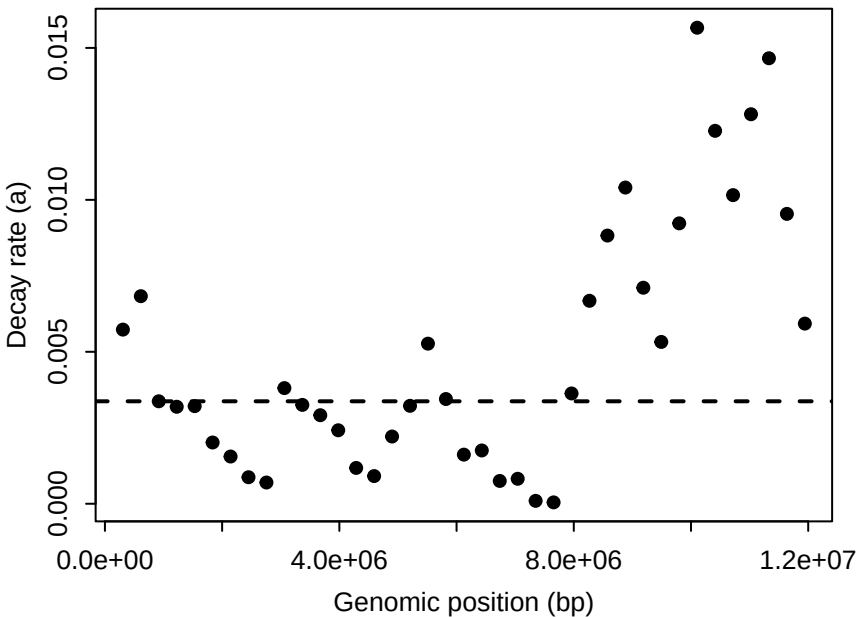
Chr5: LD contrast across windows
