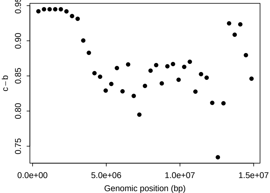
Chr14: LD contrast across windows
