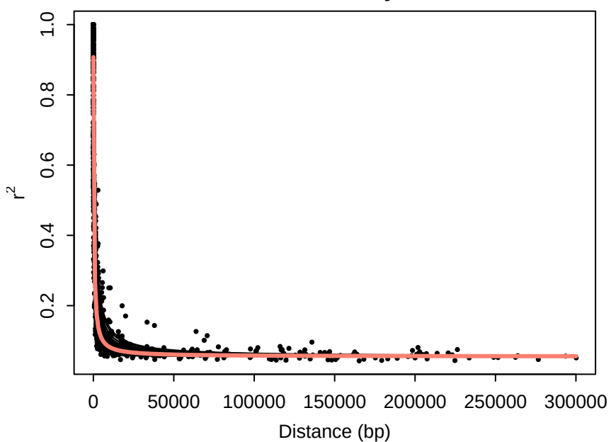
Chr16: fitted decay curves
