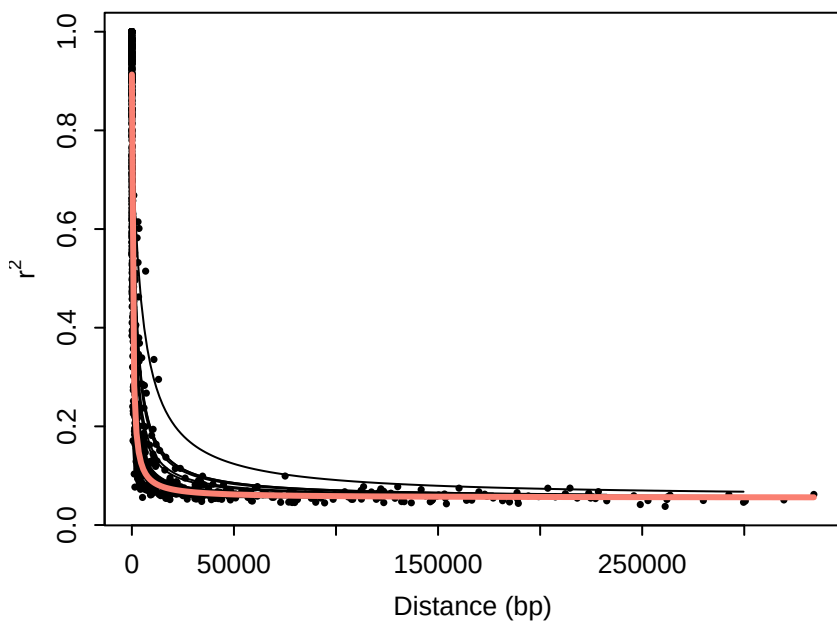
Chr12: fitted decay curves
