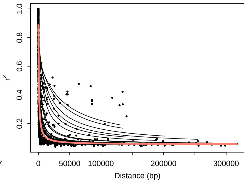
Chr9: fitted decay curves
