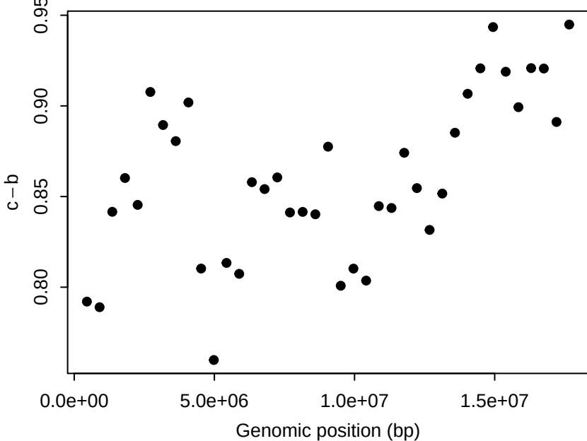
Chr16: LD contrast across windows
