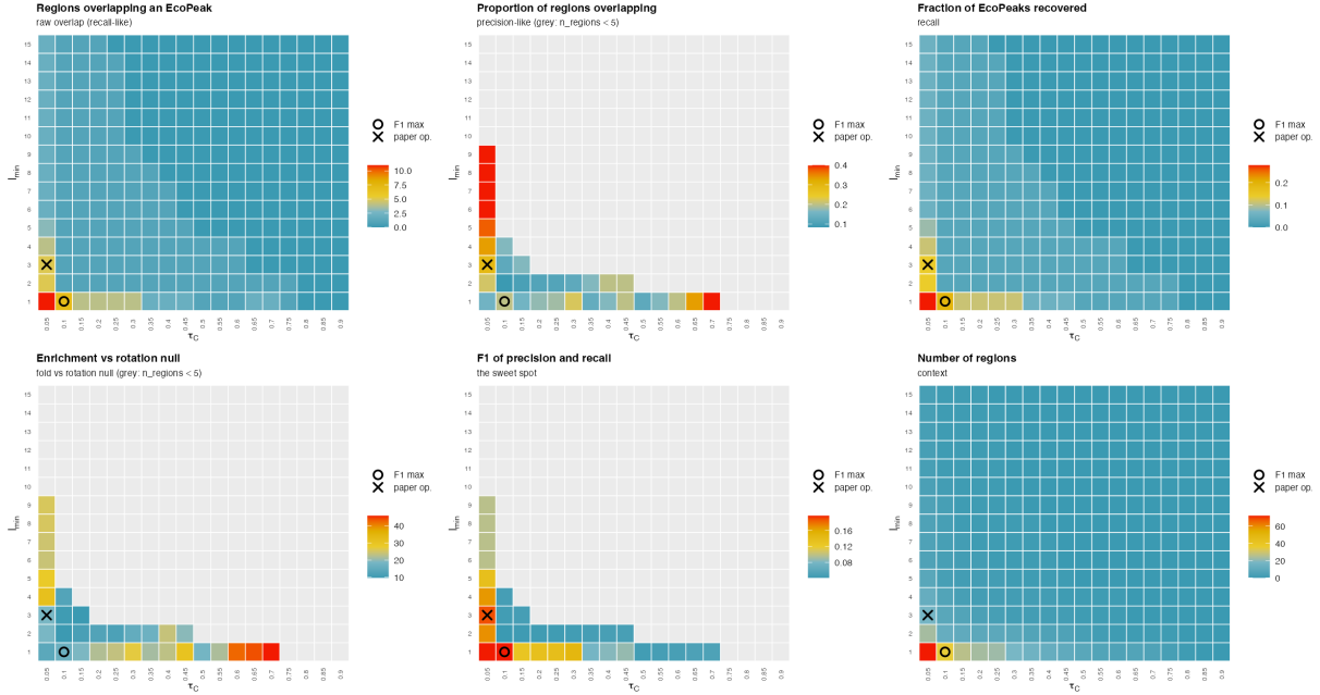
3sp EMMAX regions vs Kingman c155.specific EcoPeaks over the \tau_C \times \ell_{\min} grid
