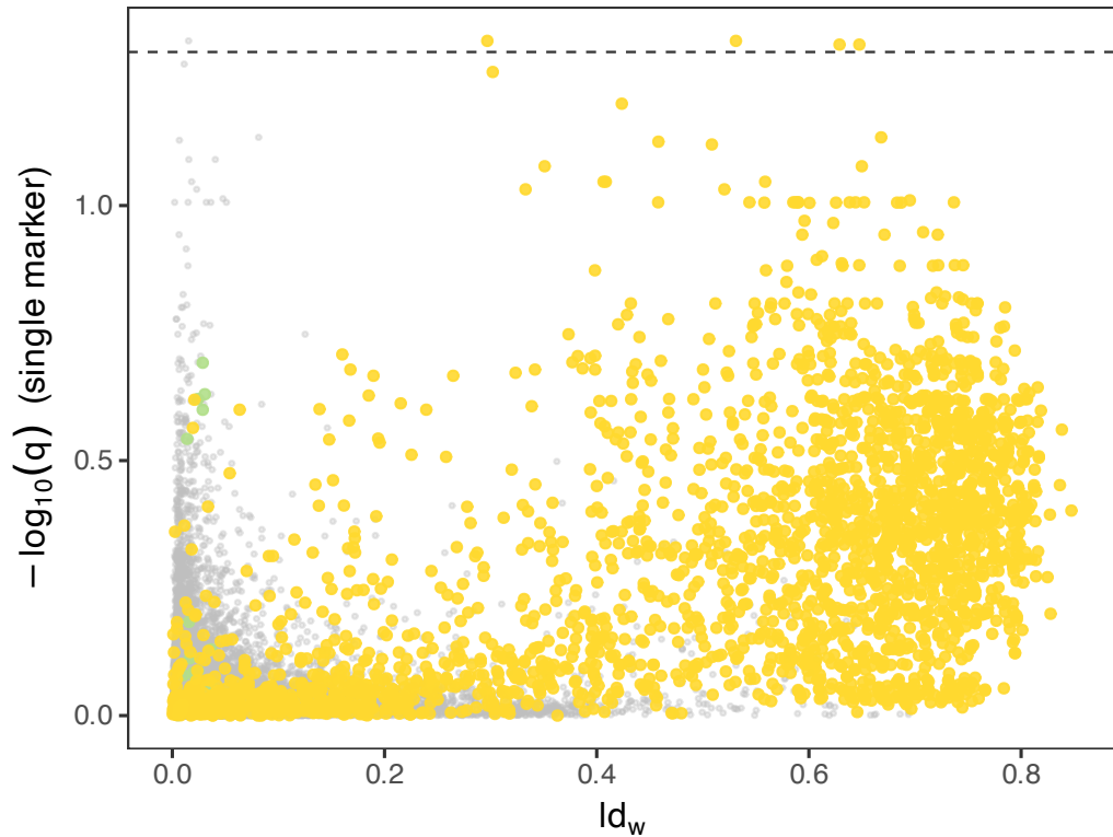
Chr1 (2 regions)
