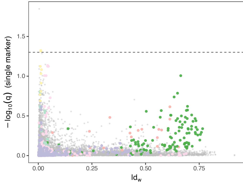
Chr4 (6 regions)
