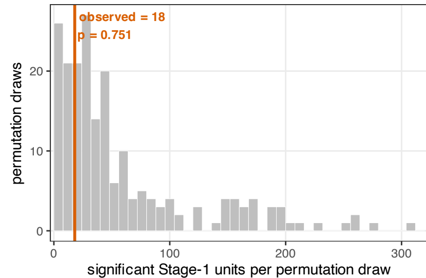
Nine-spined -- Simes
