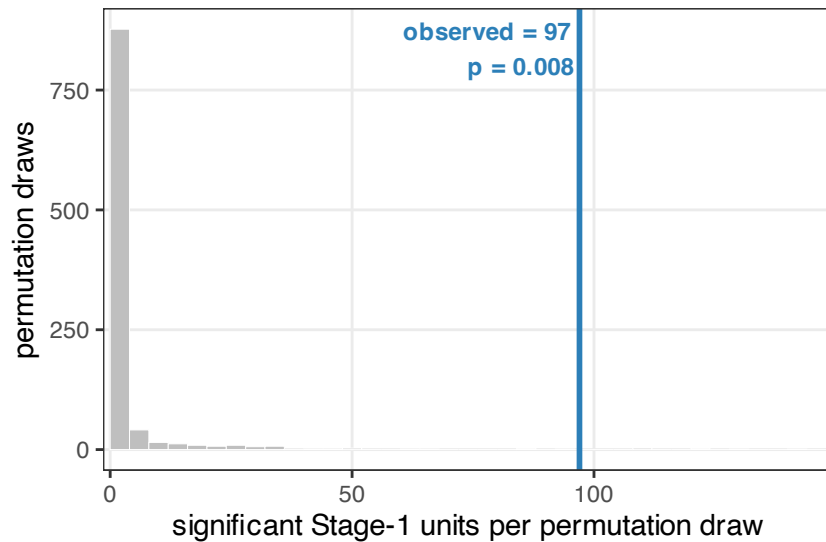
Nine-spined -- Consensus
