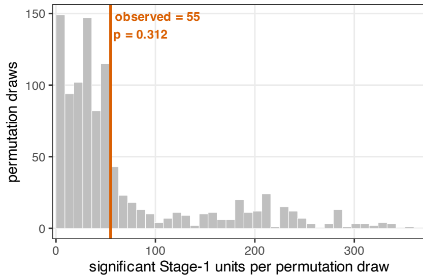
Nine-spined -- Consensus
