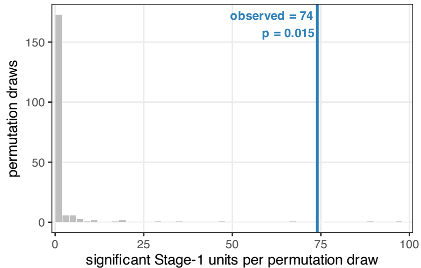
Nine-spined -- Simes
