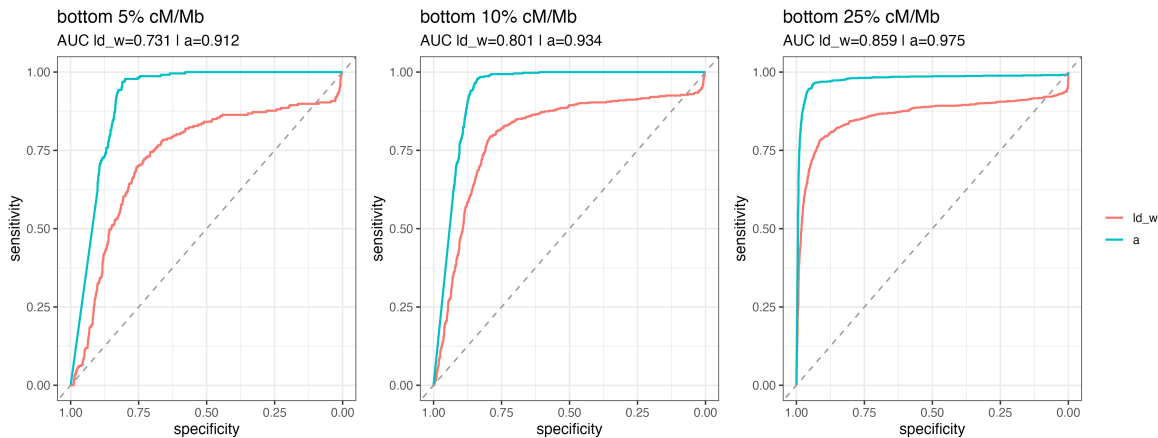
Figure S1: Discrimination of low-recombination regions by local LD support ( ld_w ) and by the window-level decay rate ( a ), against map-based recombination rate, at three definitions of “low recombination” (the lowest 5%, 10% and 25% of windows). Both are effective; the decay rate is stronger, while ld_w is defined per marker and requires no interpolation.
