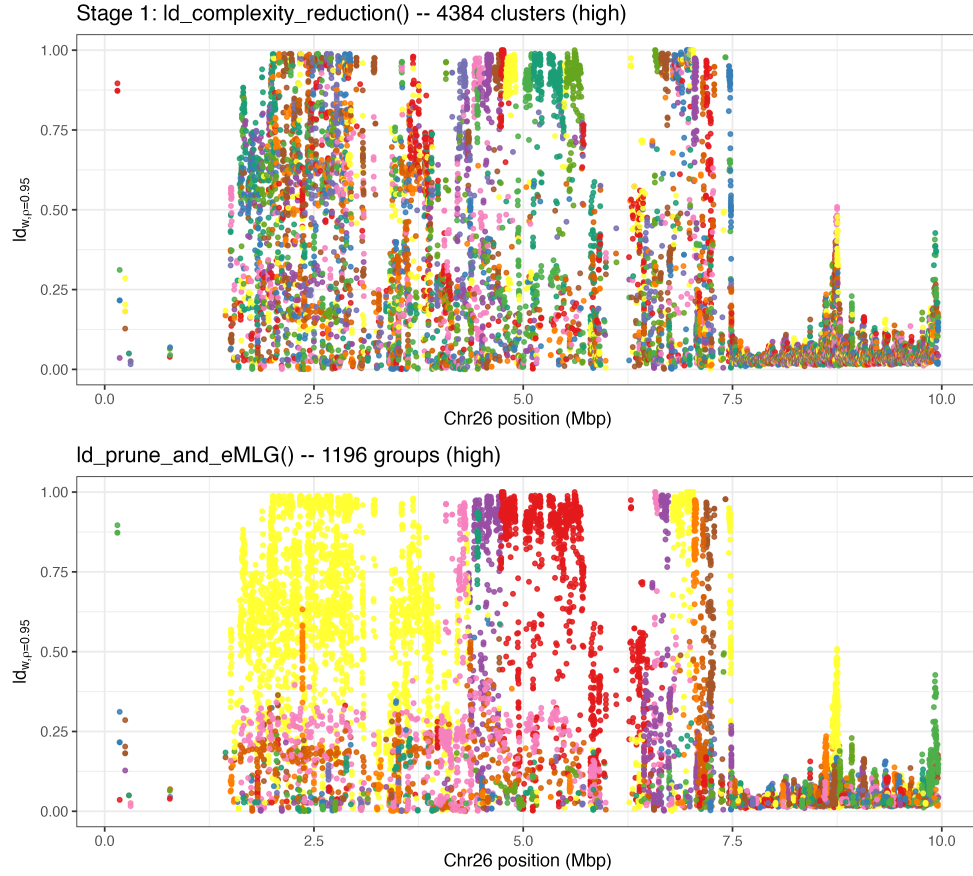
Figure S3: Stage 1 clustering compared with the combined two-stage result for Chr26, restricted to markers with high local LD support. Fragmented Stage-1 clusters within each low-recombination region are consolidated into single coherent clusters per physical LD peak, which is the intended effect of Stage 2.
