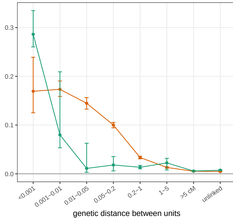
b share of the ceiling realised beyond chance
