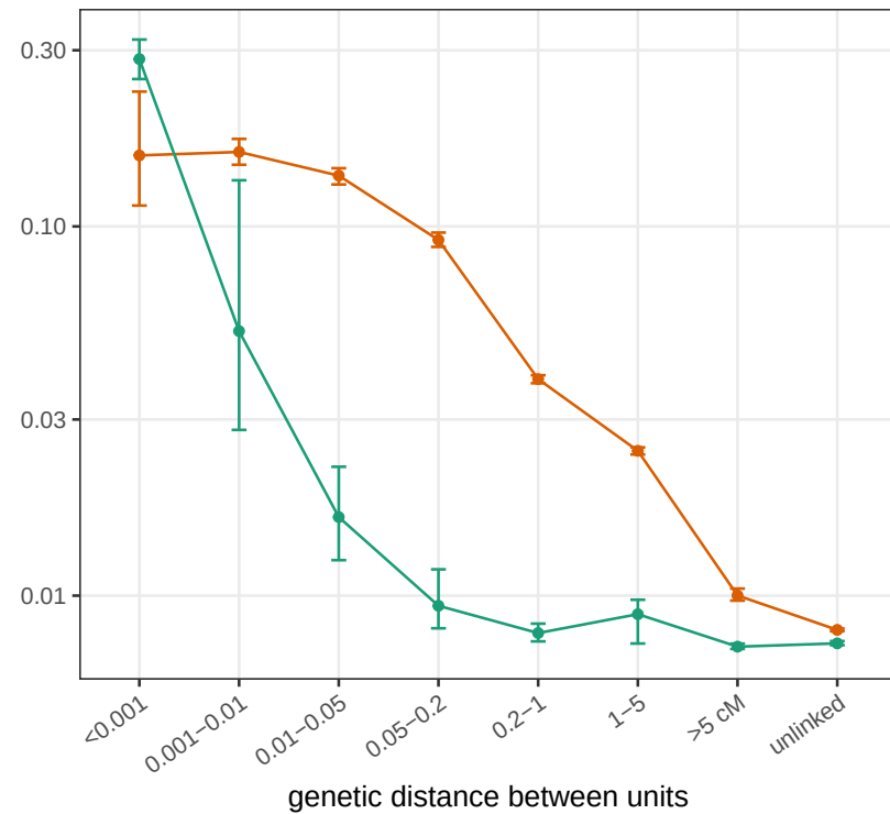
c within-population LD (log)
