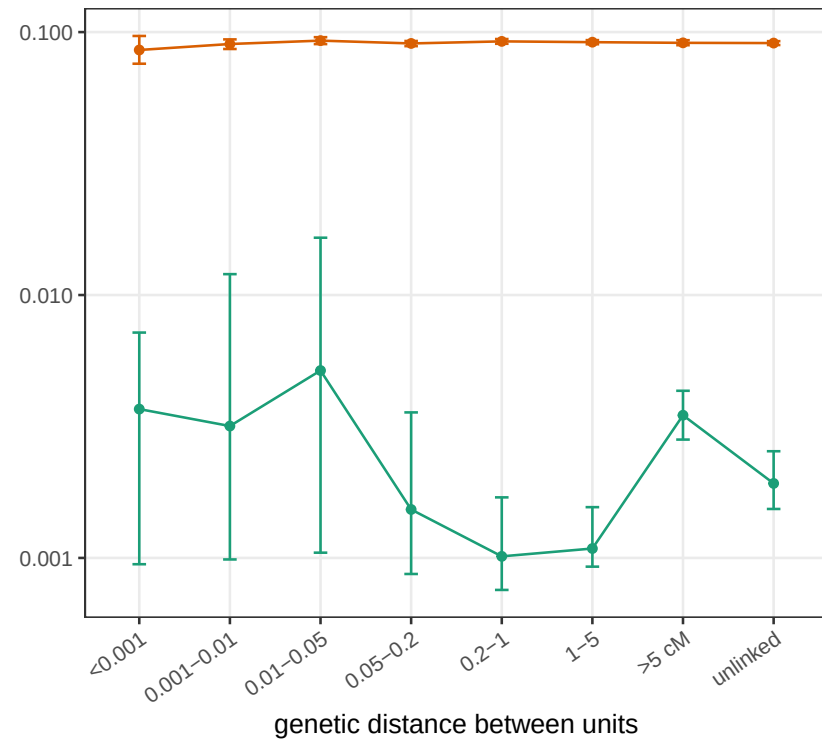
a ceiling: max among-population LD (log)
