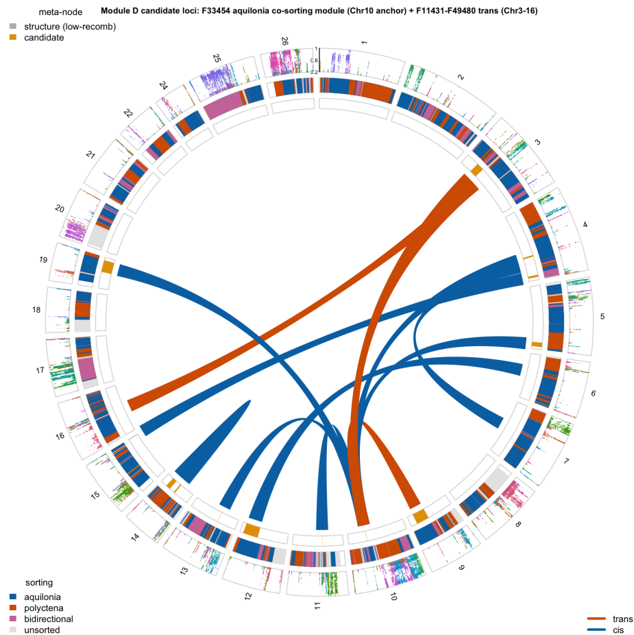
Figure 7: Genomic view of the candidate loci: each association drawn as a band spanning the full extent of the two meta-nodes it joins (cis blue, trans orange; here at full opacity as the set is sparse, with a minimum band width enforced so narrow regions stay visible). The Chr10 anchor F33454 fans out to aquilonia-sorted partners on Chr3/4/5/9/11/13/19 (bands landing on the blue aquilonia stretches of the sorting ring) – the aquilonia co-sorting module – while the single orange band F11431–F49480 (Chr3–Chr16) is the one ancestry-independent trans pair. Outer track: ld_w > 0.2 per marker; inner rings: genome-wide sorting, then the meta-node structure(grey)/candidate(gold) label.
