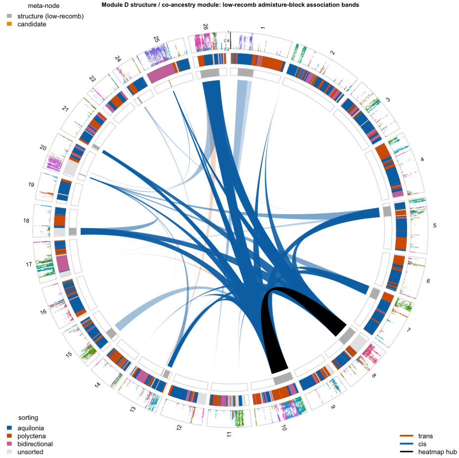
Figure 8: Genomic view of the structure / co-ancestry module (band opacity \propto degree; black = the F27700–F33095 heatmap pair). The module is almost entirely cis (blue): low-recombination admixture blocks on different chromosomes couple in the same ancestry direction, converging on the Chr8/Chr10 anchors. The contrast with Fig. 7 – cis-coupled co-ancestry here, the trans/repulsion signal with the candidates – is the visual statement that the two are different phenomena.
