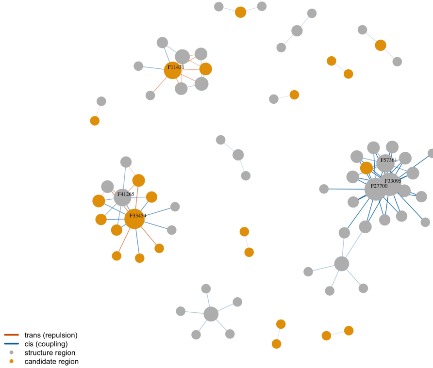
Figure 6: The Module-D meta-network after global FDR ( q < 0.01 ), paralogy removal, third-level within-region merging, and the leave-one-population-out leverage filter. Nodes are meta-nodes sized by degree; grey = low-recombination “structure” label, gold = candidate region; blue edges cis (coupling), orange edges trans (repulsion). The large grey complex (F33095/F27700/F57361) is the admixture-block structure module; the gold hub F33454 is the aquilonia co-sorting module; scattered gold–gold pairs are the pair-specific candidates.
