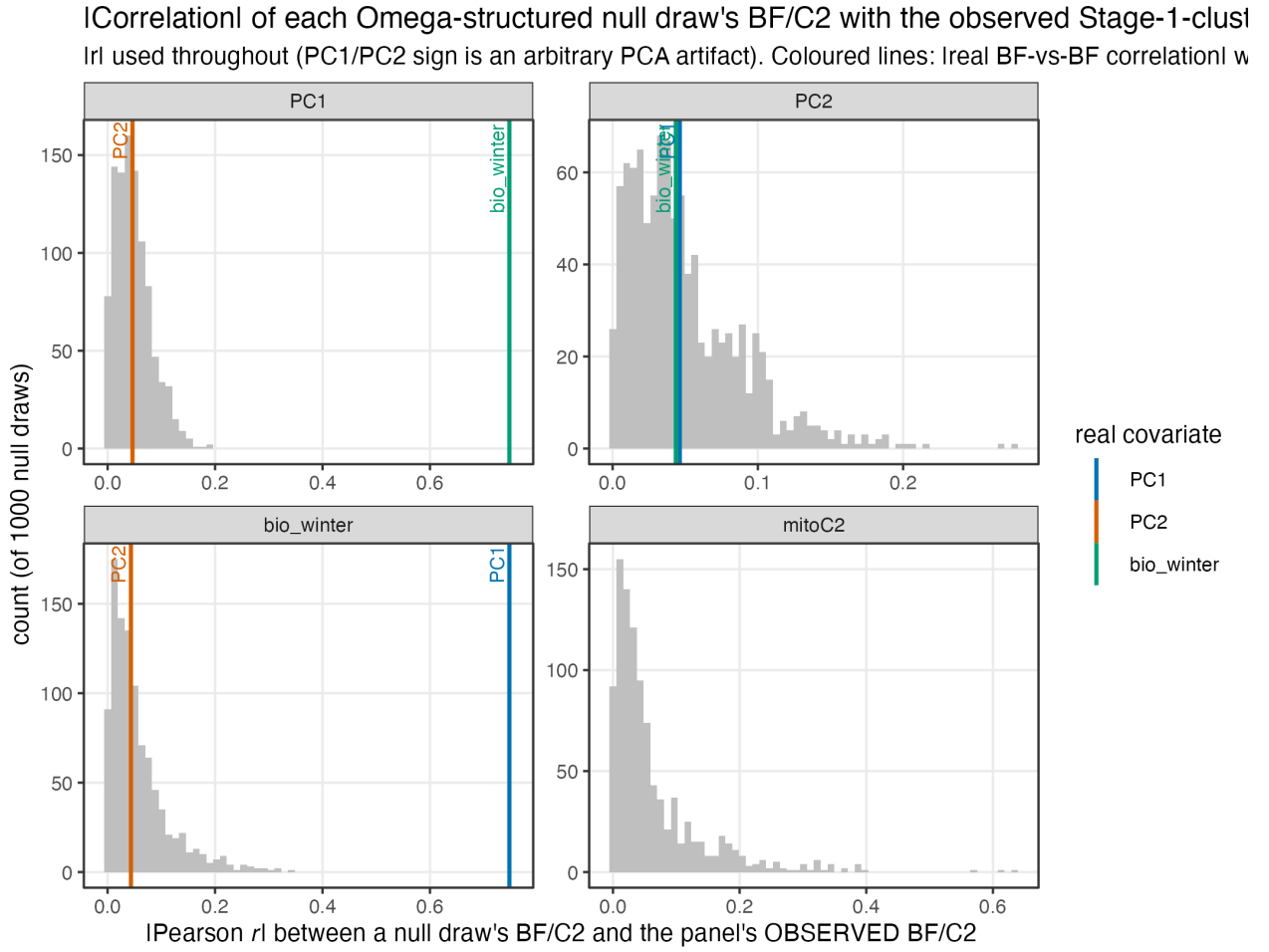
Figure 6: Grey: distribution of |r| between each of 1,000 null draws' BF/C2 and the observed BF/C2, per covariate, Stage-1-cluster resolution . Coloured vertical lines: |r| the REAL BF-vs-BF correlation between that panel's covariate and another observed covariate, same resolution. Read together with the self-consistency finding below before interpreting the PC1/bio_winter panels.
