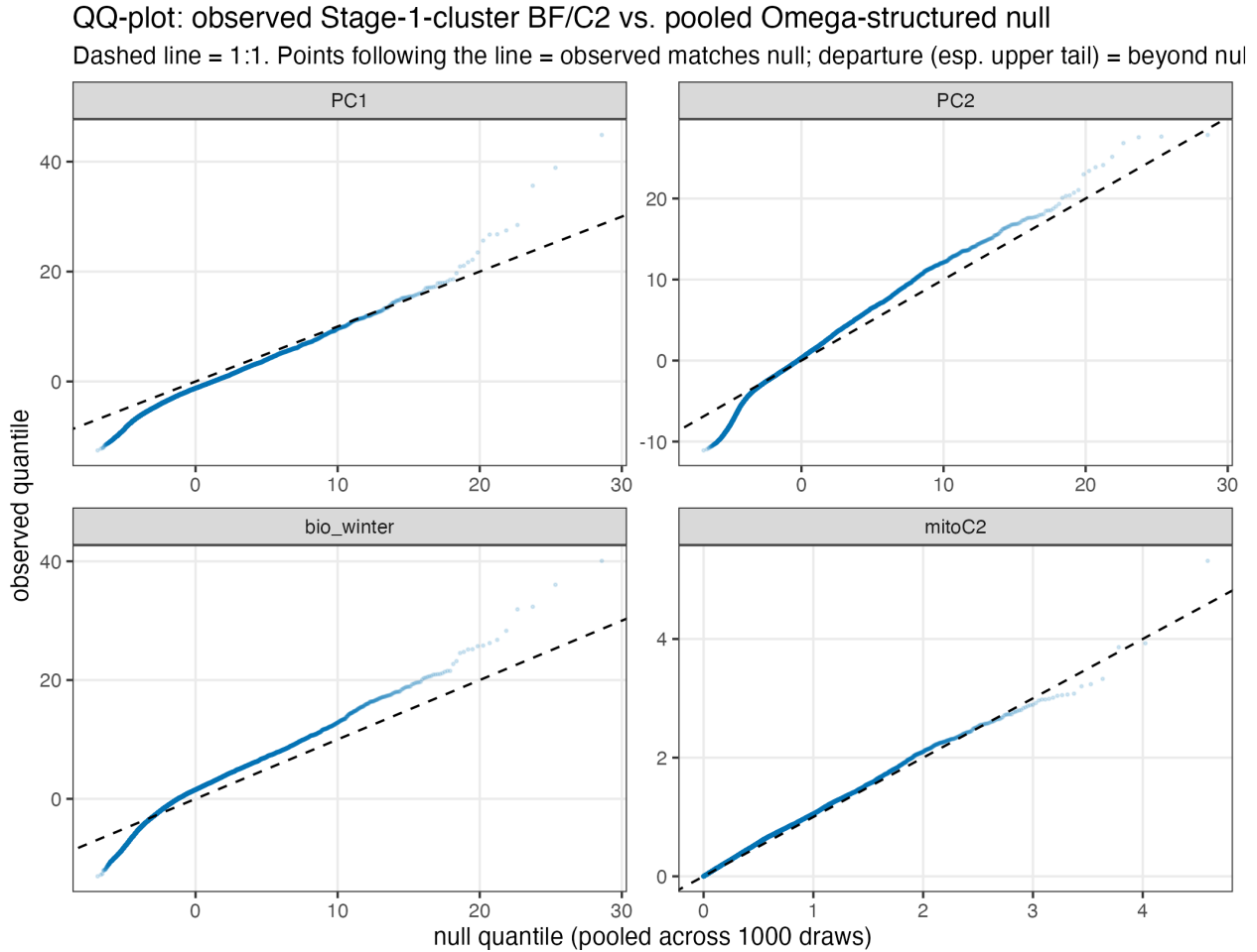
Figure 7: QQ-plots, observed vs. pooled null (1,000 draws), Stage-1- cluster resolution. Dashed line = 1:1.
