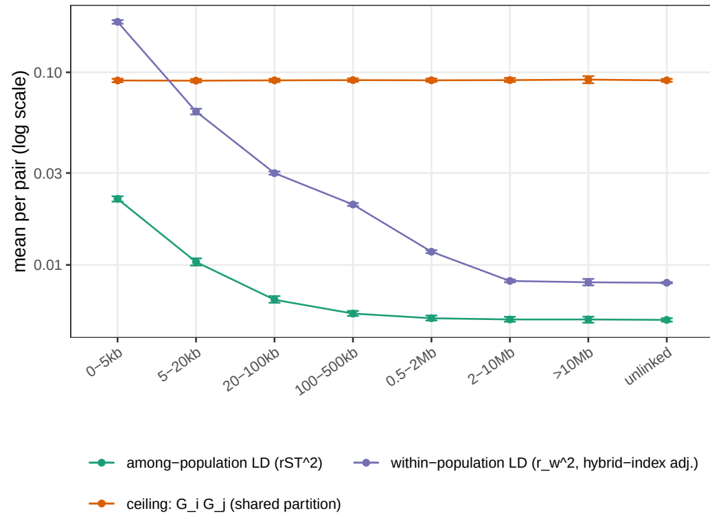
a LD components vs distance
