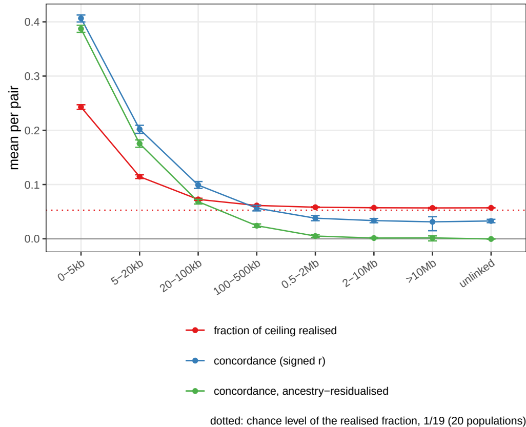
b shared partitions vs distance
