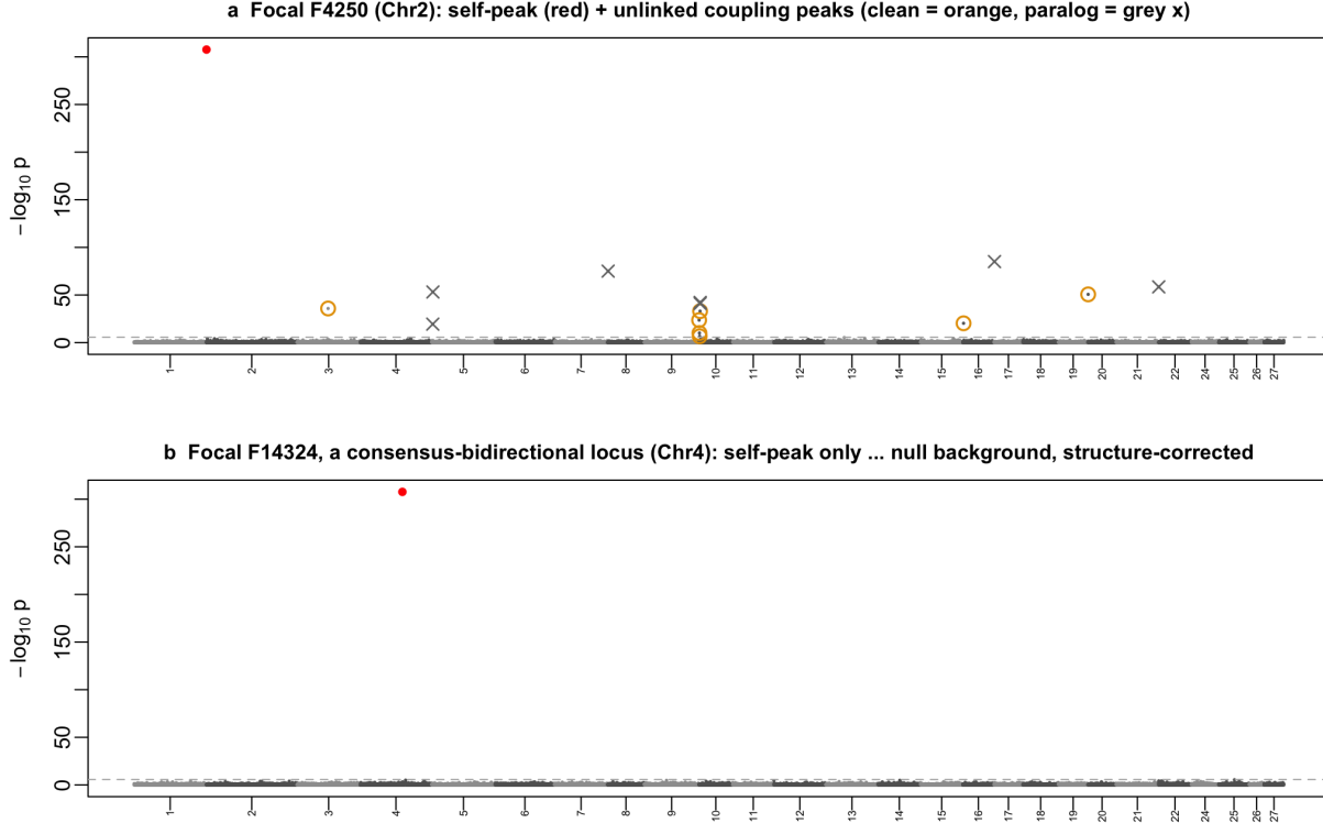
Figure 1: Structure-corrected two-locus association (EMMAX, double leave-one-chromosome-out K from the differentiated eMLGs). (a) A focal locus (F4250, Chr2) showing its self-peak (red) and unlinked partner peaks, split by the paralogy filter into genuine candidates (orange) and cross-chromosome duplicates (grey crosses). (b) A consensus-bidirectional focal locus (F14324, Chr4): only its self-peak, a flat structure-corrected background ( \lambda \approx 1 ). Dashed line: Bonferroni threshold.
