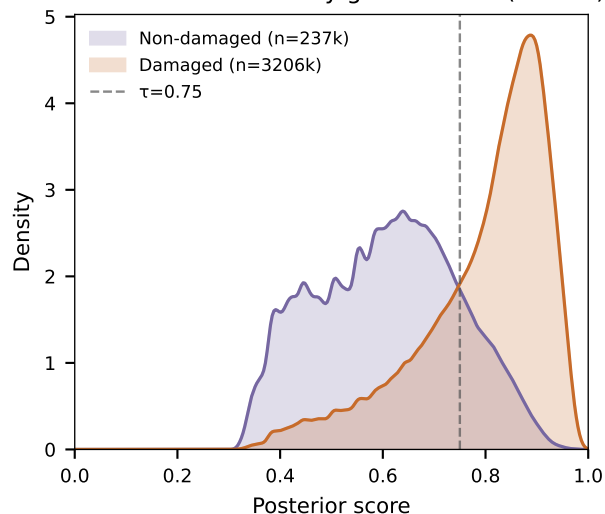
B. Score distribution by ground truth (AT-rich)
