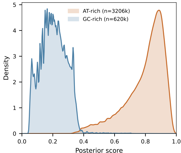
A. Score distribution by sample type (damaged reads)
