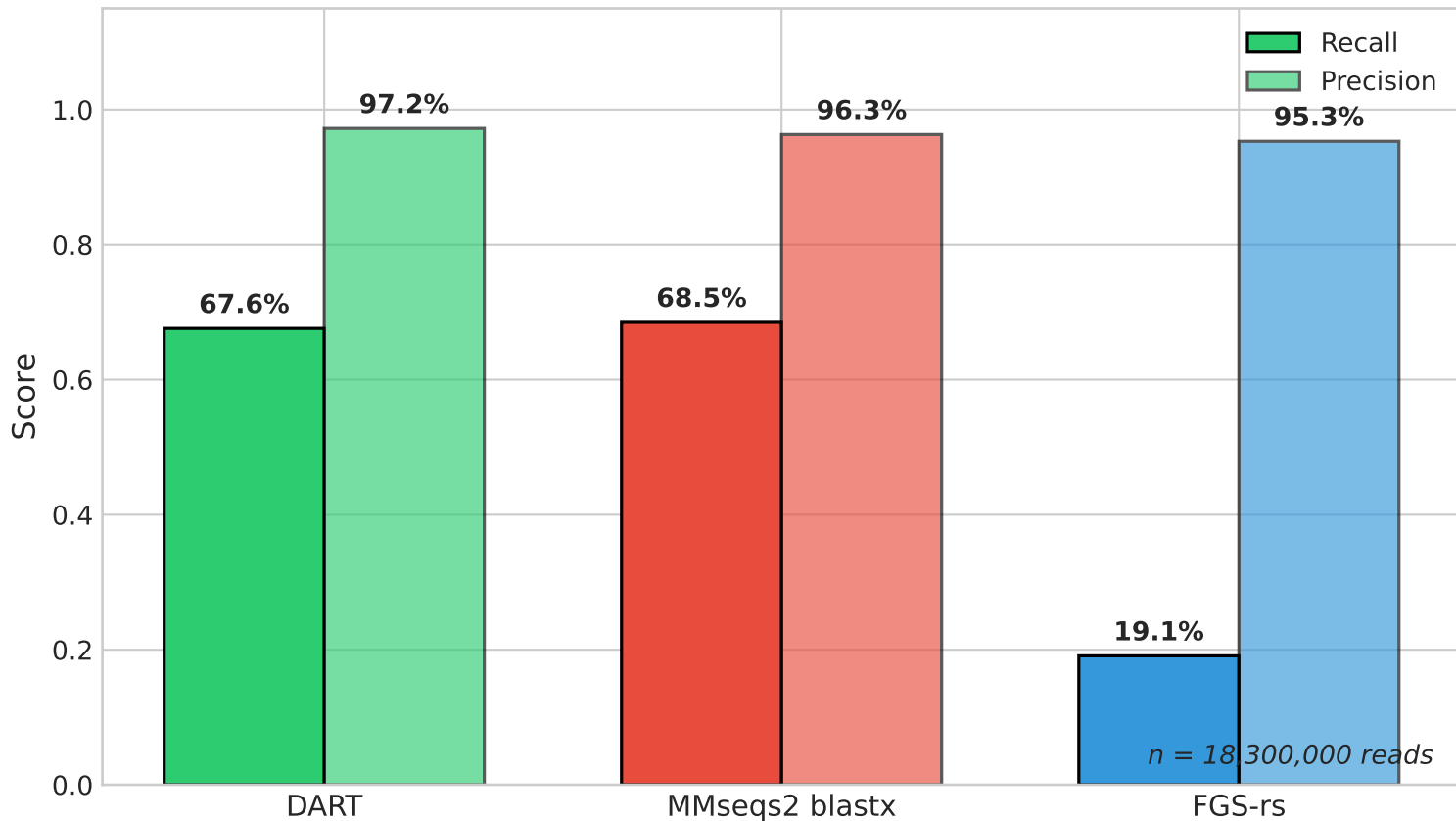
Gene prediction method comparison ( \geq 90\% identity match to ground-truth proteins, 18.3M synthetic ancient reads)
