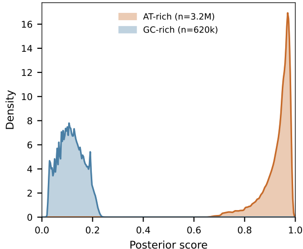
A. Score distribution by sample type (damaged reads)
