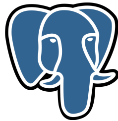
Figura 22: Logo Postgres
