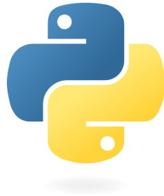
Figura 21: Logo Python
