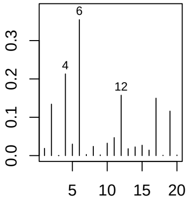
Cook's distance
