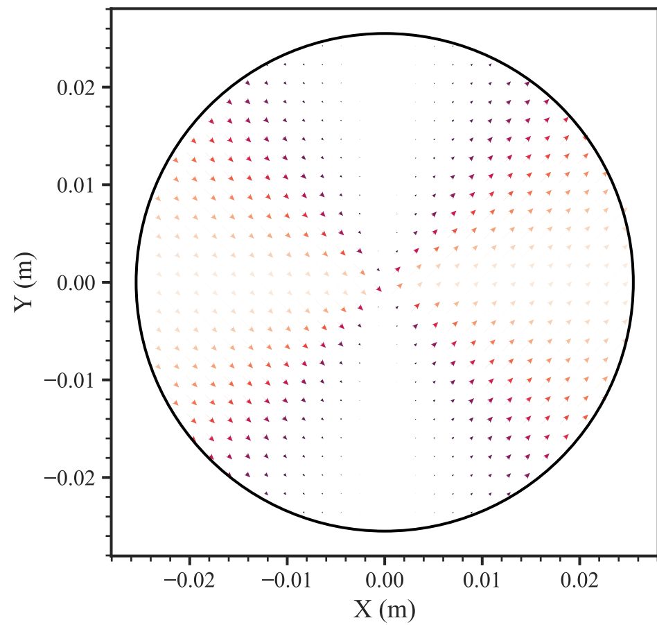
Augen Gneiss ( 90.0^\circ ) — principal tensile strain proxy
