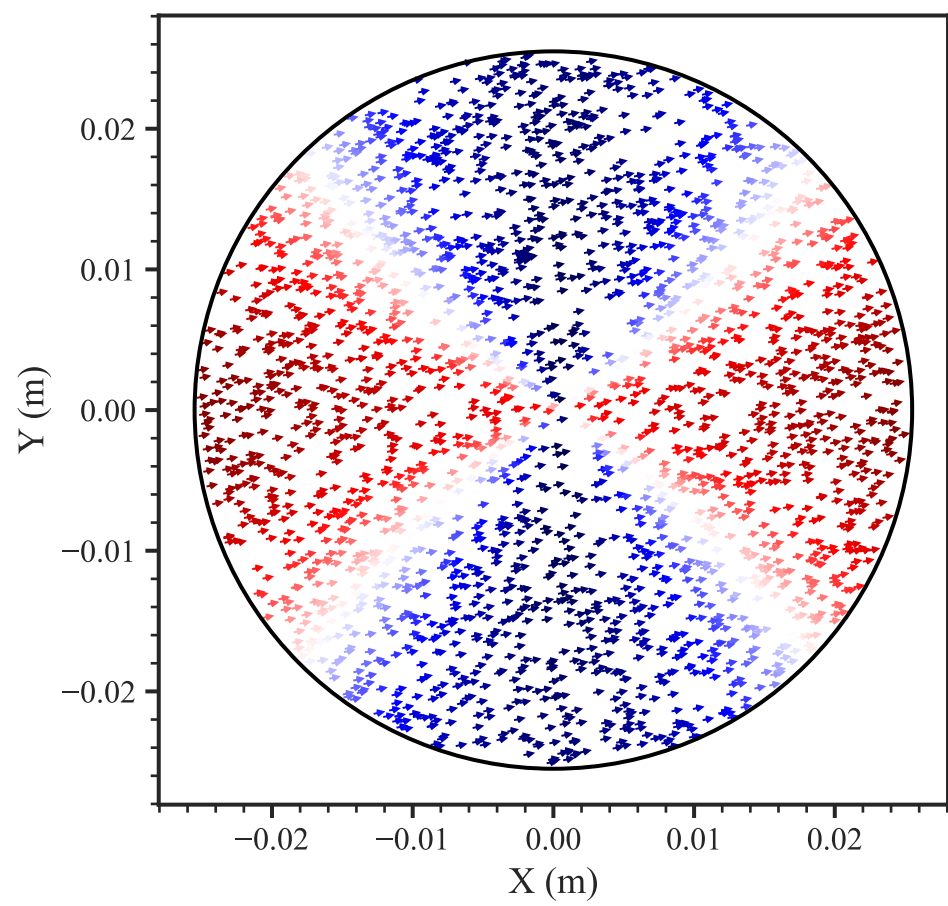
Augen Gneiss (45°)
