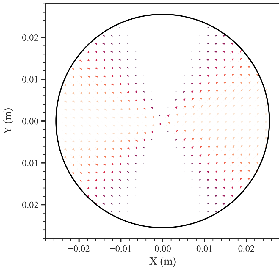
Augen Gneiss ( 75.0^\circ ) — principal tensile strain proxy
