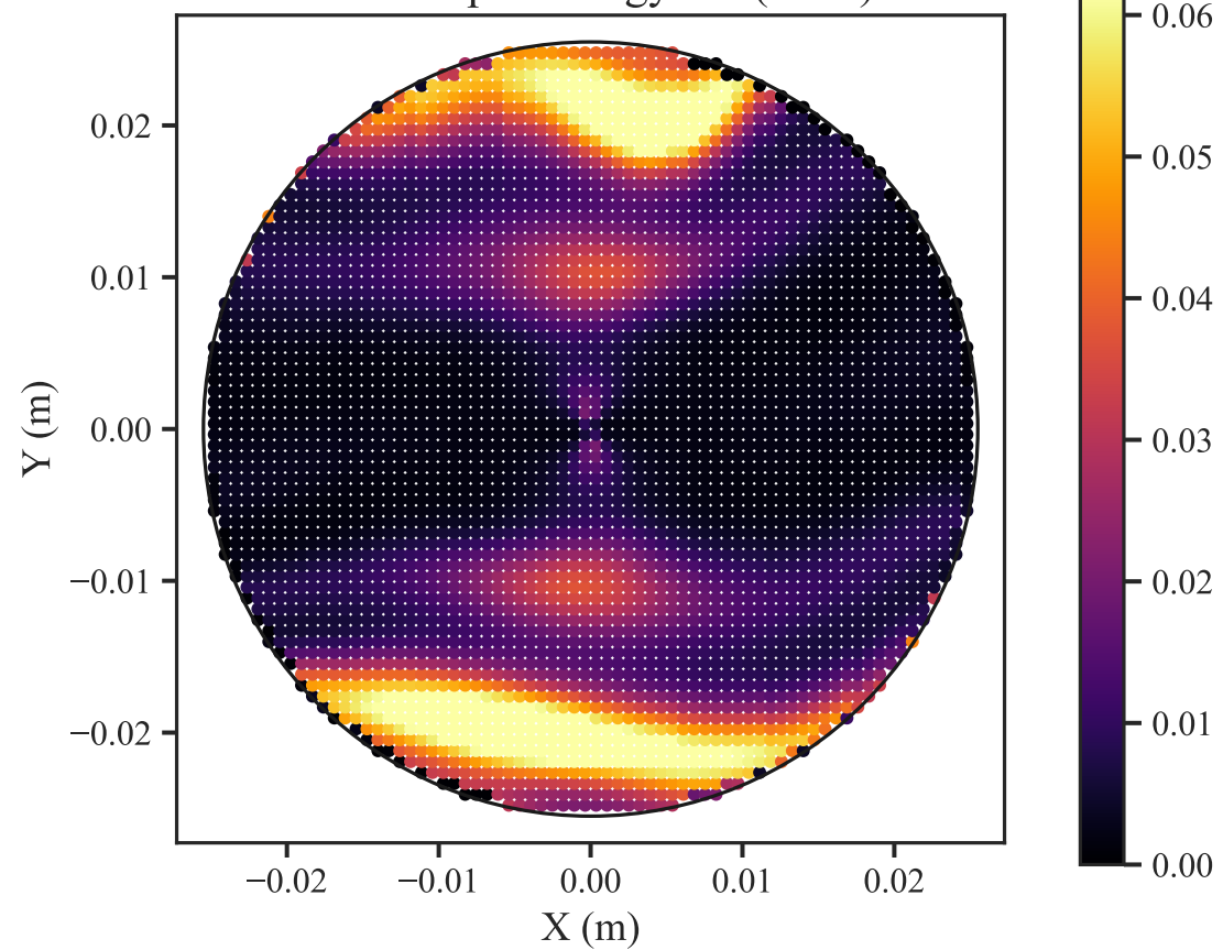
Orthotropic Energy U^* ( \theta=0^\circ )
