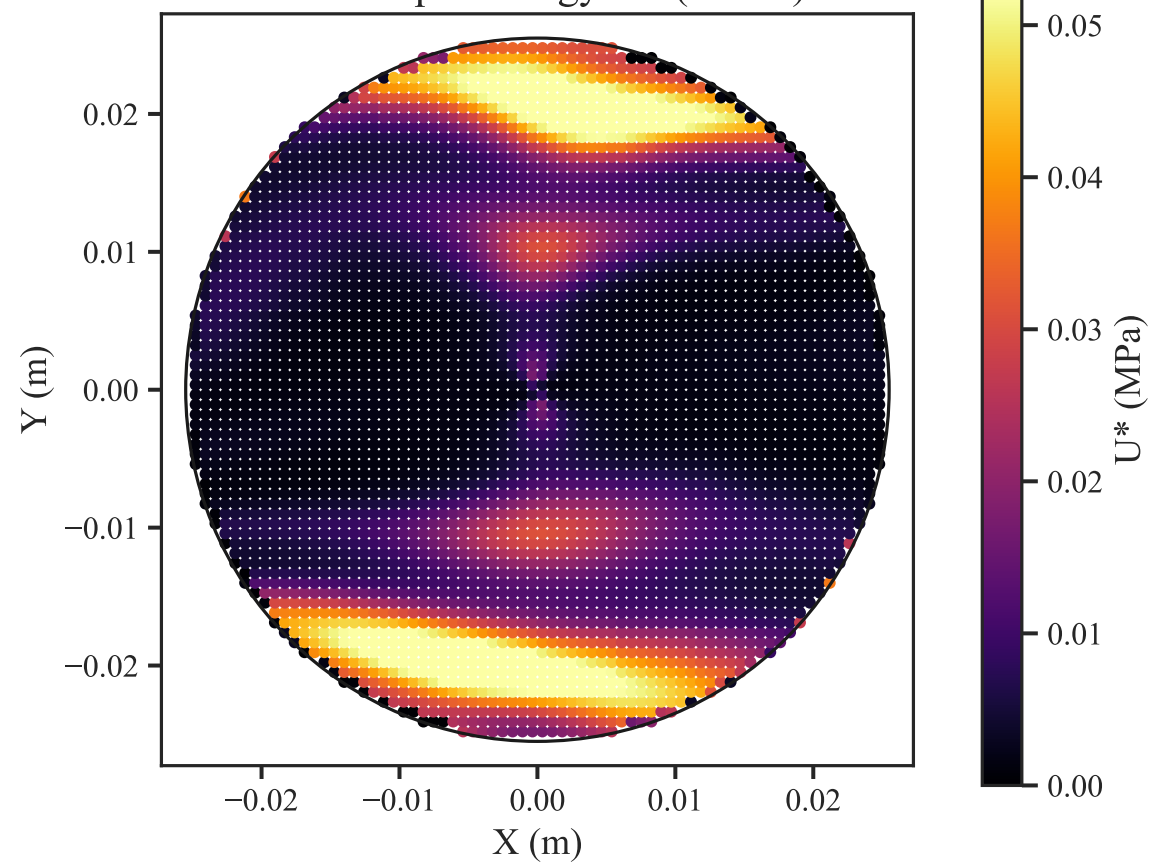
Orthotropic Energy U^* ( \theta=15^\circ )
