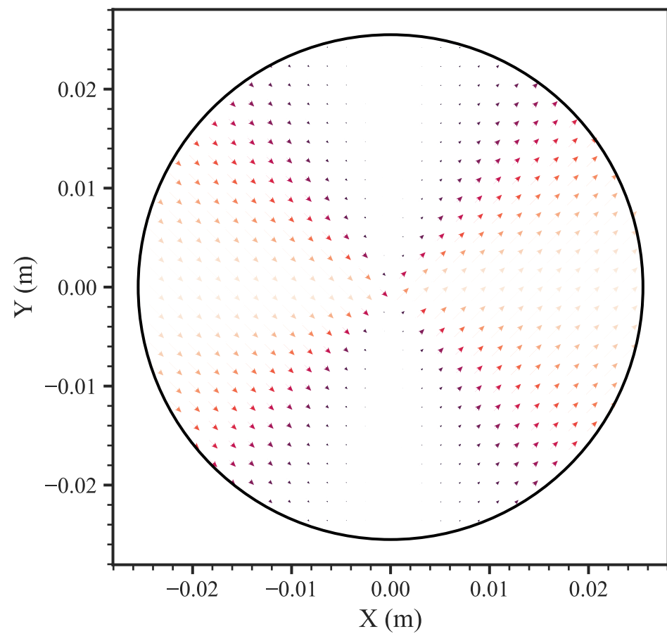
Augen Gneiss (60.0°) — principal tensile strain proxy
