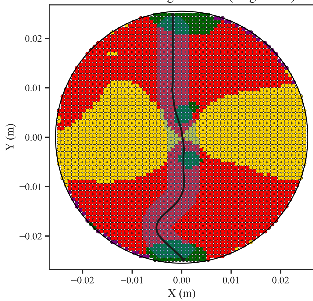
Failure Modes: Augen Gneiss (Angle: 45°)
