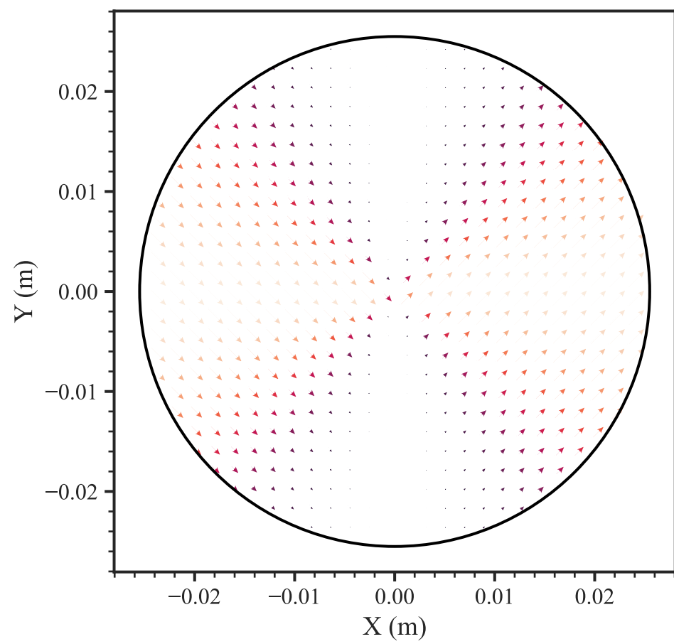
Augen Gneiss ( 30.0^\circ ) — principal tensile strain proxy
