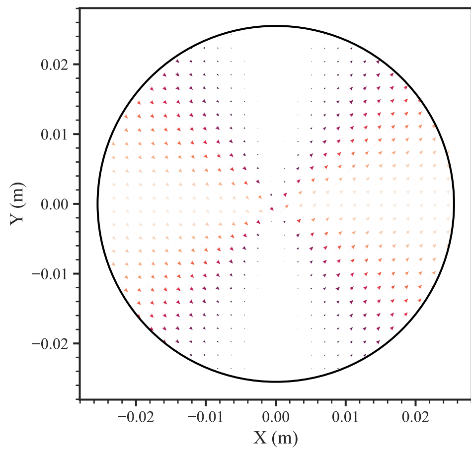
Augen Gneiss (90.0°) — principal tensile strain proxy
