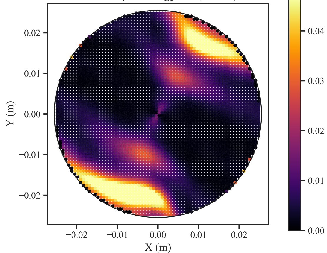
Orthotropic Energy U^* ( \theta=30^\circ )
