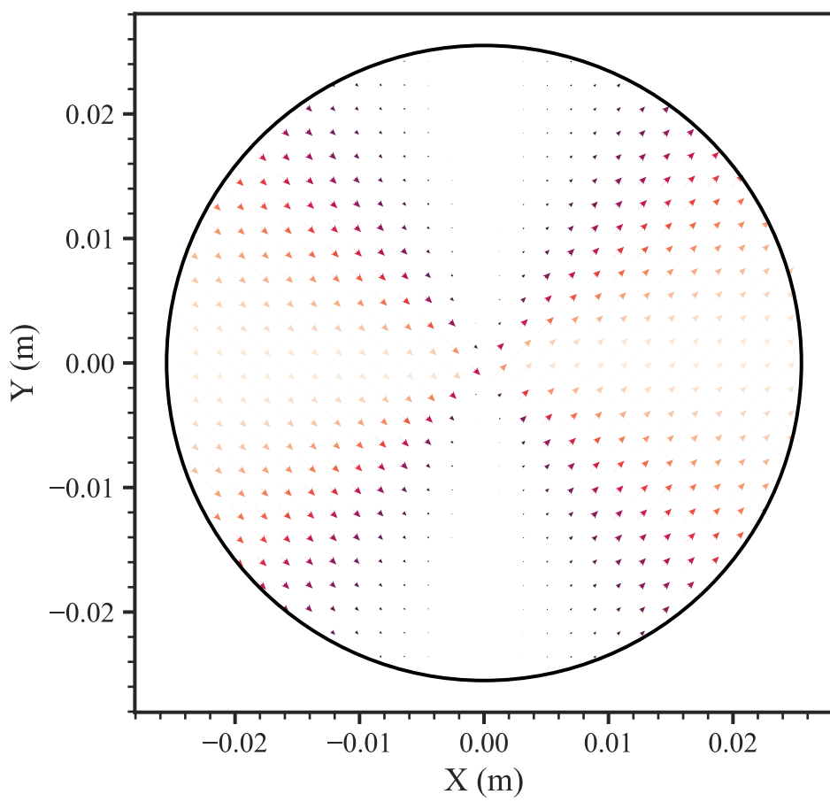
Augen Gneiss ( 45.0^\circ ) — principal tensile strain proxy
