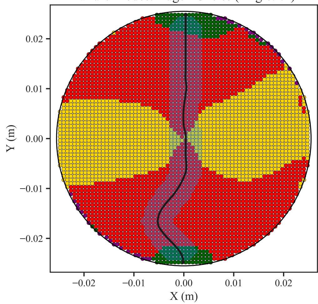
Failure Modes: Augen Gneiss (Angle: 30°)
