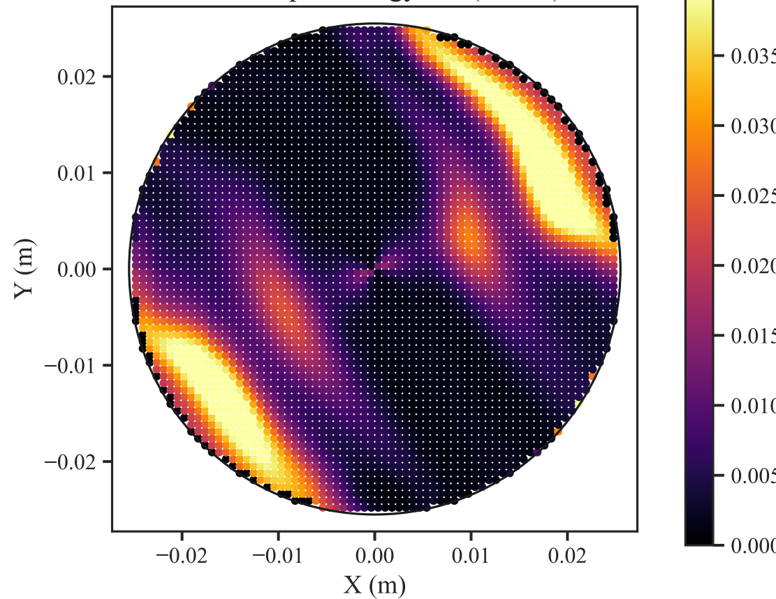
Orthotropic Energy U^* ( \theta=60^\circ )
