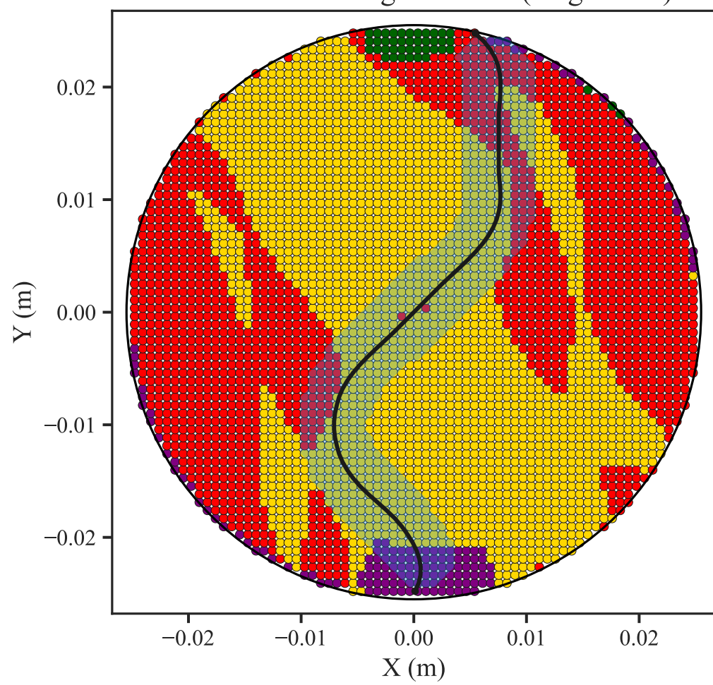
Failure Modes: Augen Gneiss (Angle: 75°)
