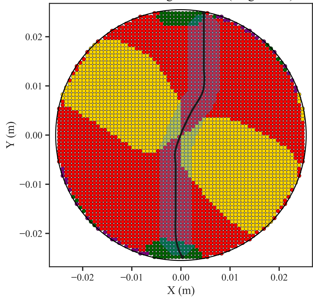
Failure Modes: Augen Gneiss (Angle: 60°)
