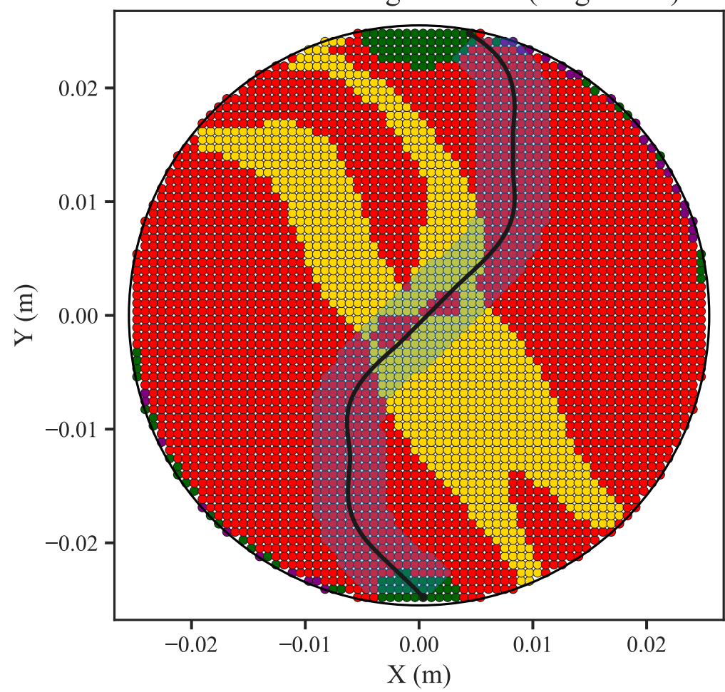
Failure Modes: Augen Gneiss (Angle: 90°)
