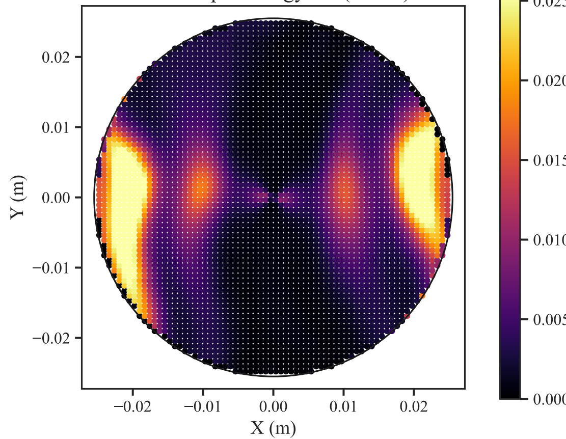
Orthotropic Energy U^* ( \theta=90^\circ )
