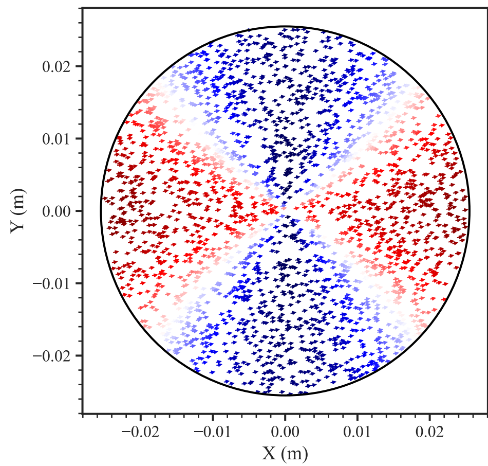
Augen Gneiss (30°)
