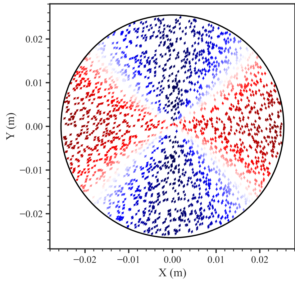
Augen Gneiss (90°)
