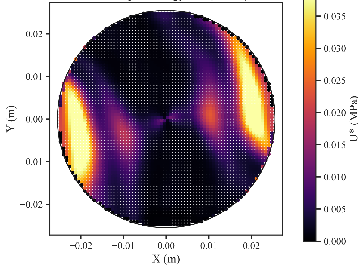
Orthotropic Energy U^* ( \theta=75^\circ )
