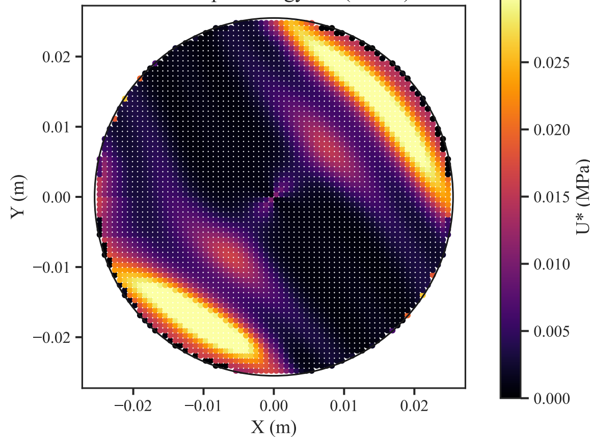
Orthotropic Energy U^* ( \theta=45^\circ )
