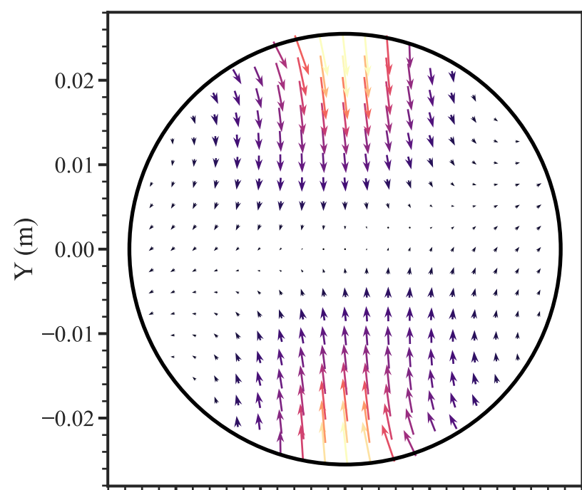
Augen Gneiss (90°)
