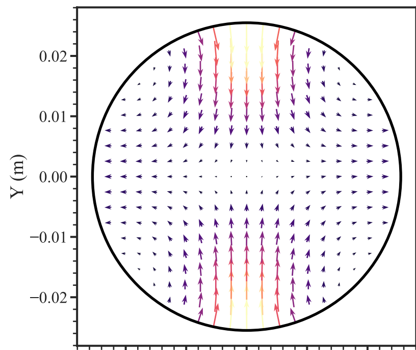
Augen Gneiss (30°)
