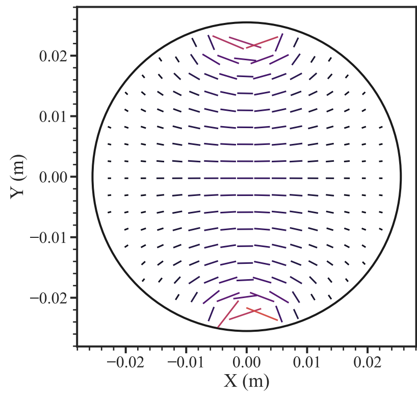
Augen Gneiss (90°) — \sigma_1 +/ E_{eff} axis
