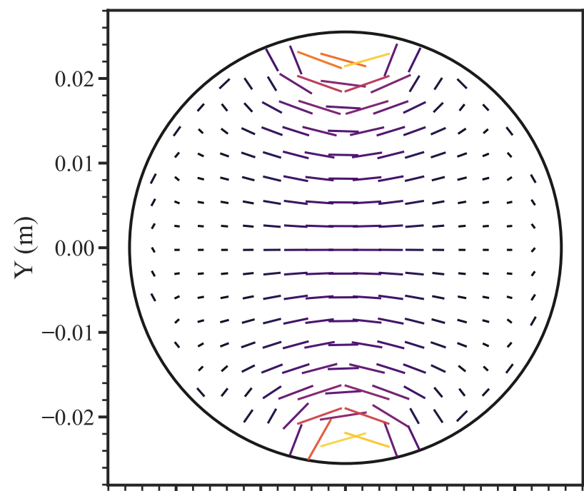
Augen Gneiss (30°) — \sigma_1 +/ E_{eff} axis
