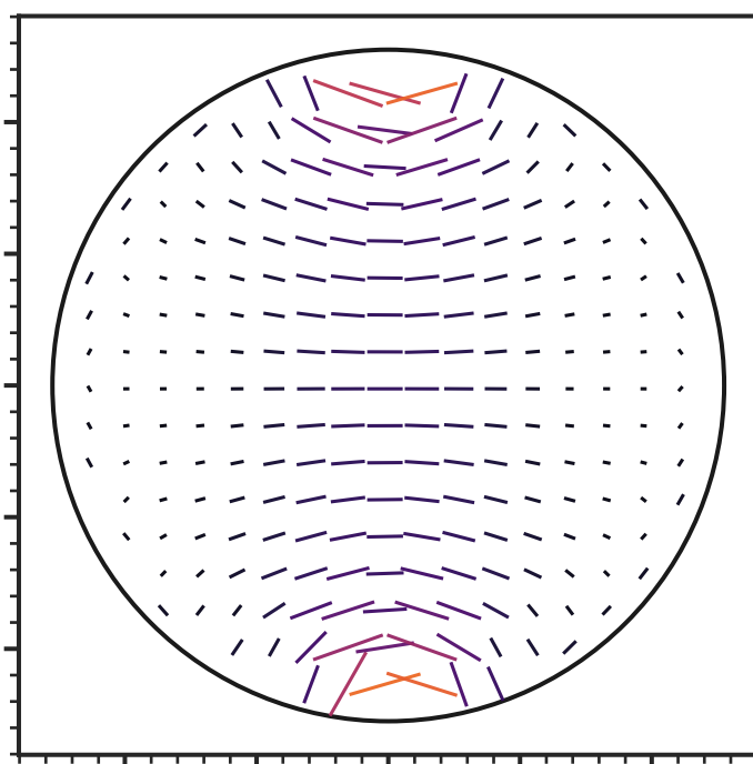
Augen Gneiss (45°) — \sigma_1 +/ E_{eff} axis
