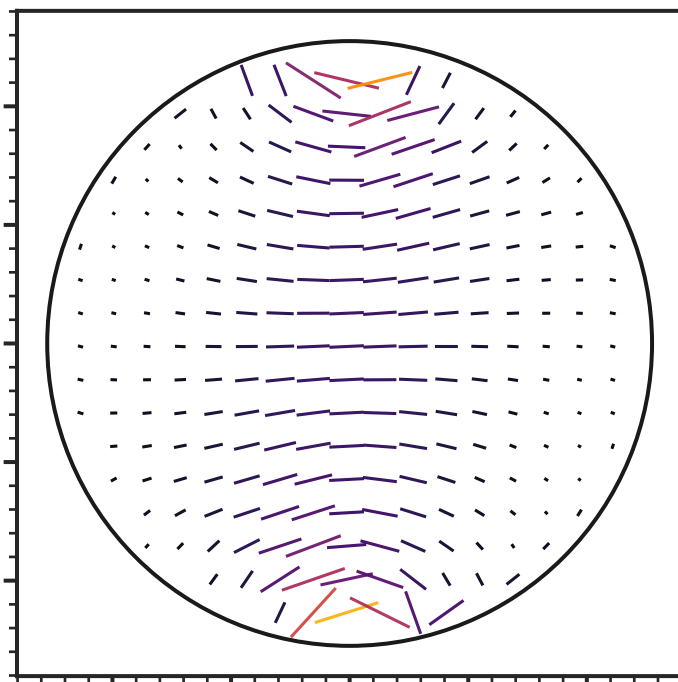
Augen Gneiss (75°) — \sigma_1 +/ E_{eff} axis
