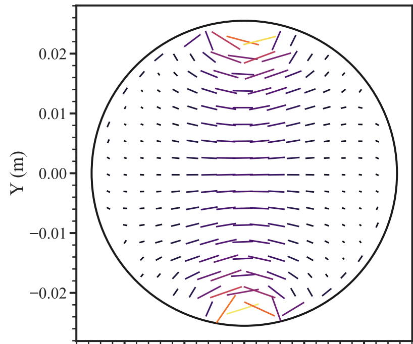
Augen Gneiss (60°) — \sigma_1 +/ E_{eff} axis
