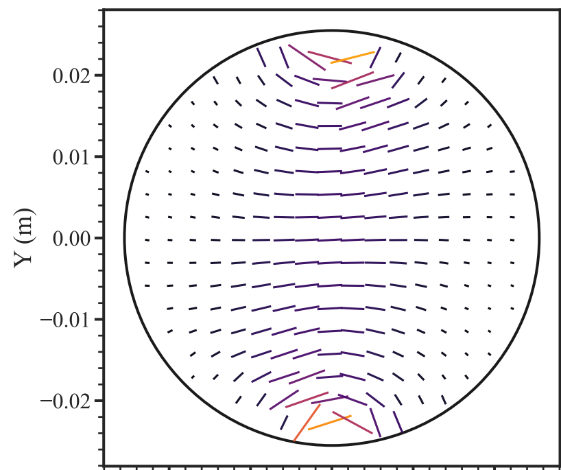
Augen Gneiss (90°) — \sigma_1 +/ E_{eff} axis
