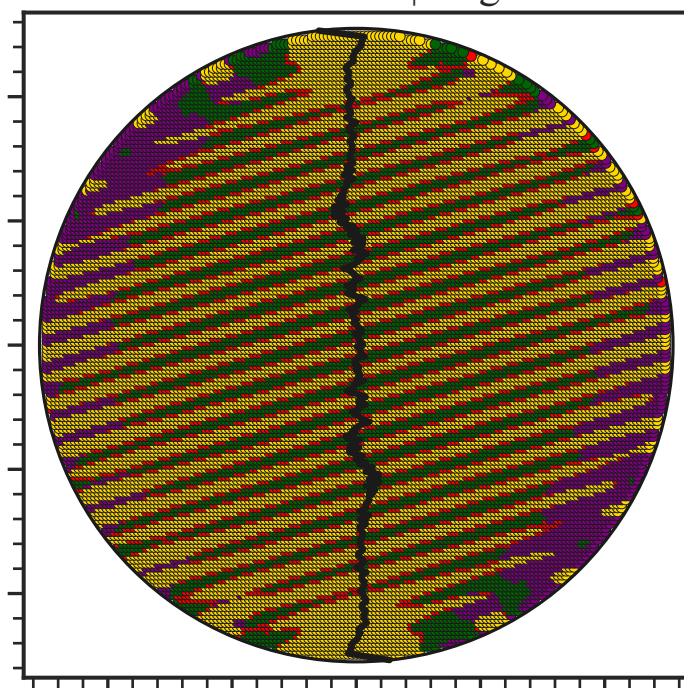
Psammatic Schist | Angle=45°
