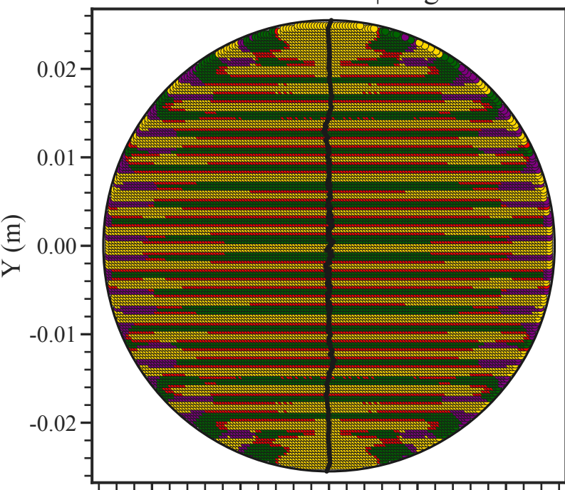
Psammatic Schist | Angle=30°
