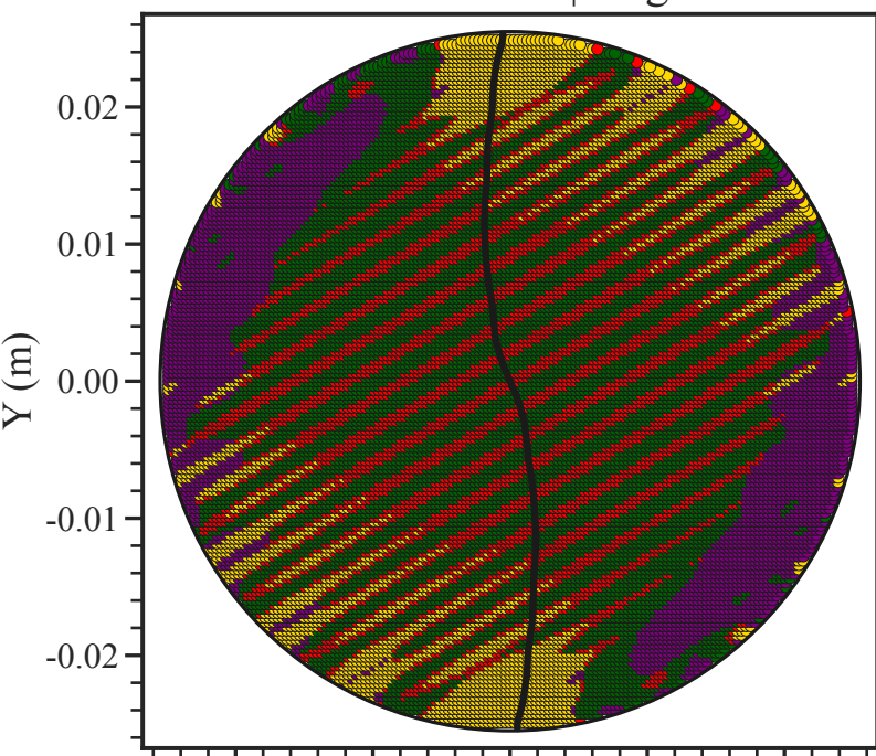
Psammatic Schist | Angle=60°
