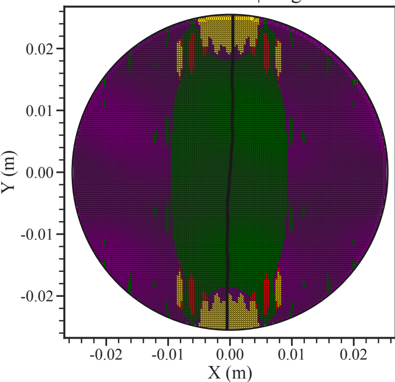
Psammatic Schist | Angle=90°
