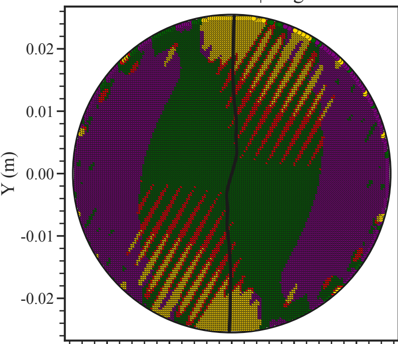
Psammatic Schist | Angle=90°
