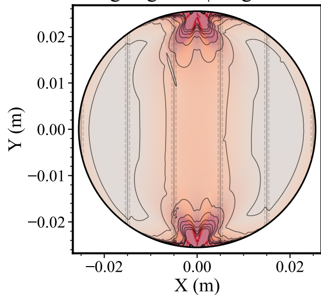
Augen gneiss | Angle=90°
