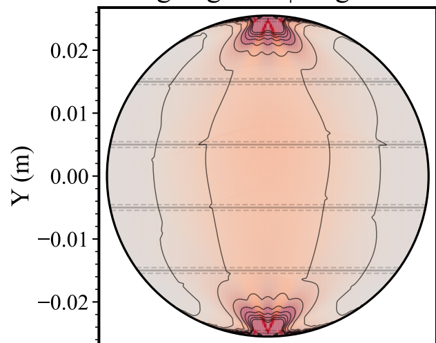
Augen gneiss | Angle=30°
