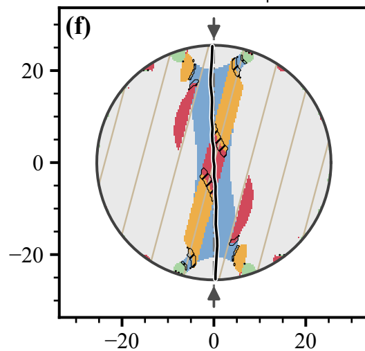
Augen gneiss, \alpha_{\text{exp}} = 75^\circ
