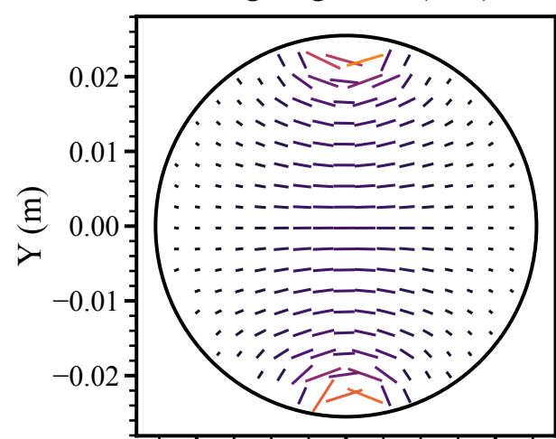
Augen gneiss (60°)
