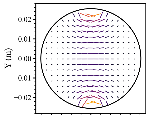
Augen gneiss (0°)
