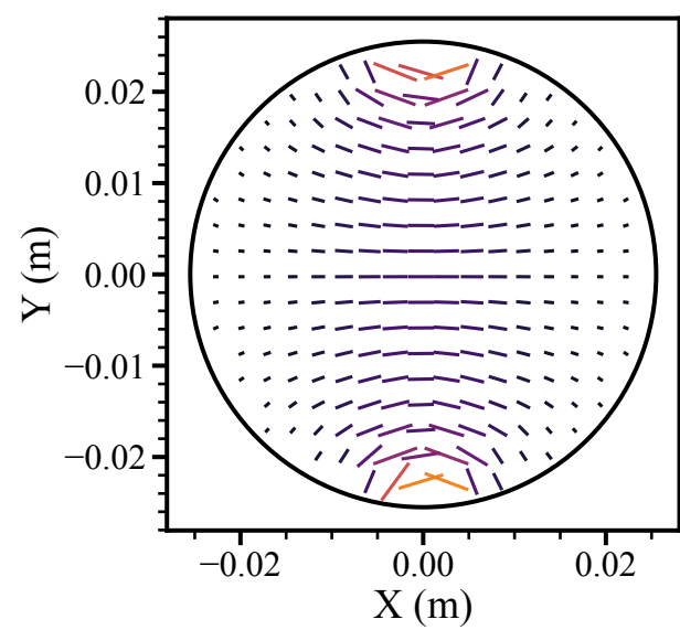
Augen gneiss (90°)
