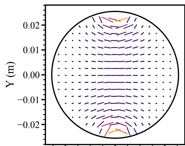
Augen gneiss (30°)
