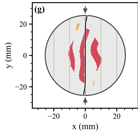
Augen gneiss, \alpha = 90^\circ
