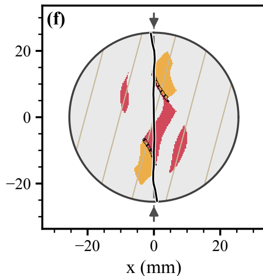
Augen gneiss, \alpha = 75^\circ
