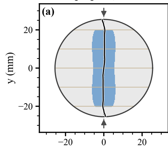
Augen gneiss, \alpha = 0^\circ
