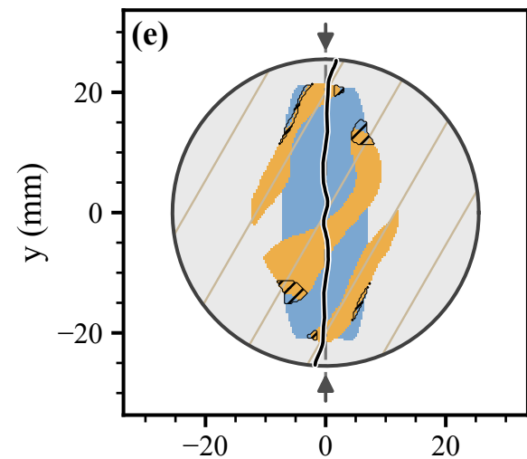
Augen gneiss, \alpha = 60^\circ
