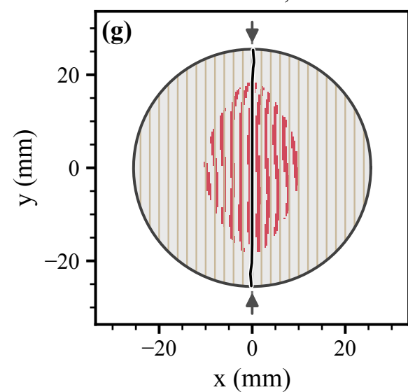
Psammitic schist, \alpha = 90^\circ
