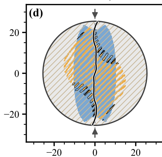
Psammitic schist, \alpha = 45^\circ
