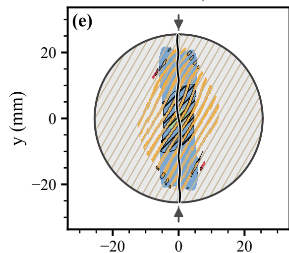
Psammitic schist, \alpha = 60^\circ
