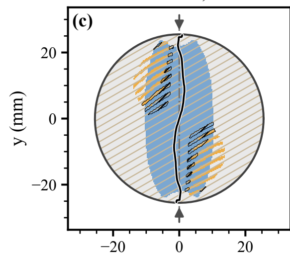
Psammitic schist, \alpha = 30^\circ
