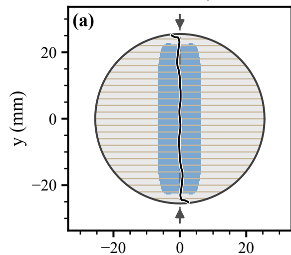
Psammitic schist, \alpha = 0^\circ
