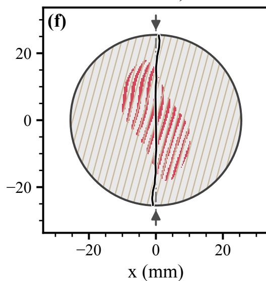
Psammitic schist, \alpha = 75^\circ
