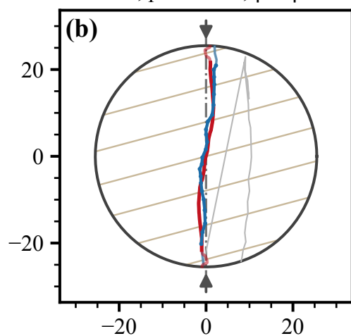
Psammitic schist, \alpha = 45^\circ obs 92.0^\circ , pred 90.6^\circ , |\Delta\theta| = 1.4^\circ
