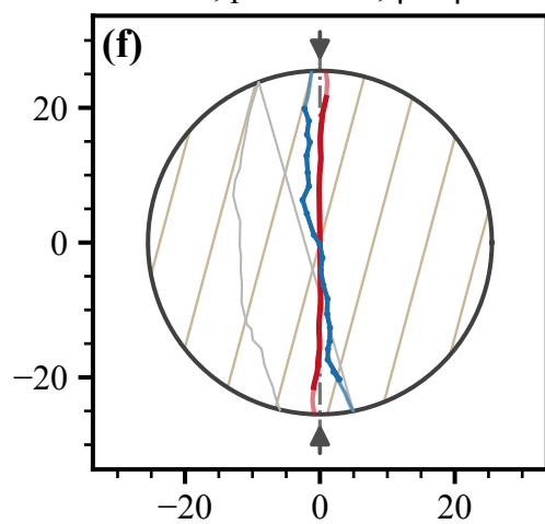
Psammitic schist, \alpha = 75^\circ obs 96.7^\circ , pred 89.1^\circ , |\Delta\theta| = 7.6^\circ
