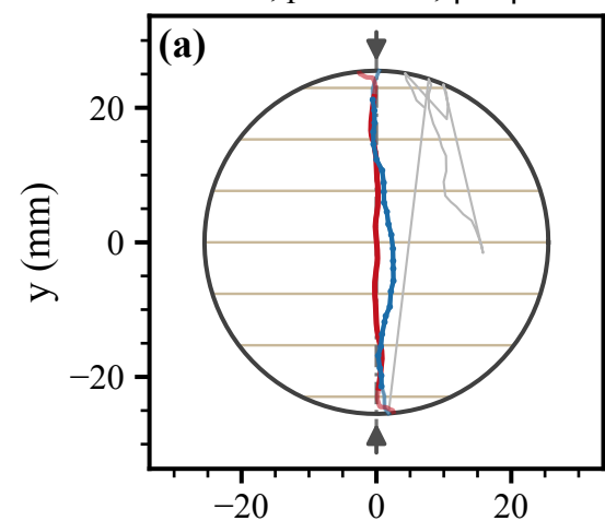
Psammitic schist, \alpha = 30^\circ obs 86.0^\circ , pred 86.8^\circ , |\Delta\theta| = 0.8^\circ
