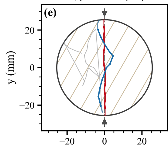
Psammitic schist, \alpha = 90^\circ obs 92.6^\circ , pred 89.9^\circ , |\Delta\theta| = 2.7^\circ
