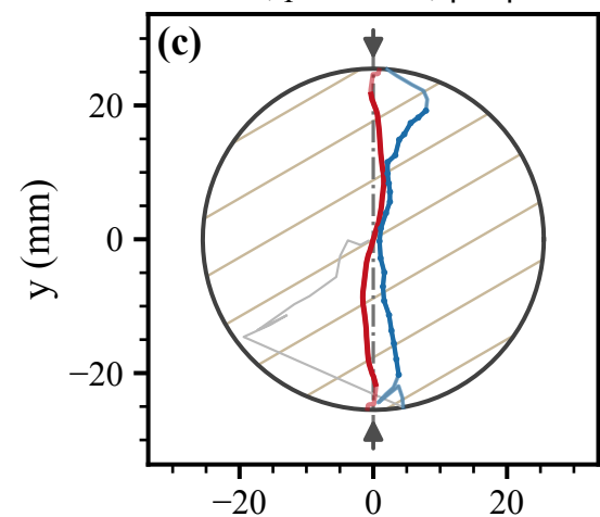
Psammitic schist, \alpha = 60^\circ obs 87.1^\circ , pred 90.9^\circ , |\Delta\theta| = 3.8^\circ
