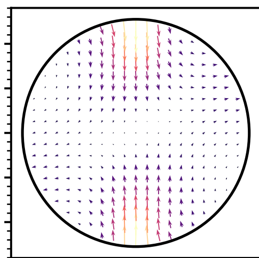
Psammitic schist (45°)
