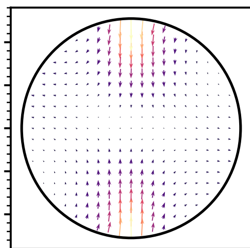
Psammitic schist (75°)
