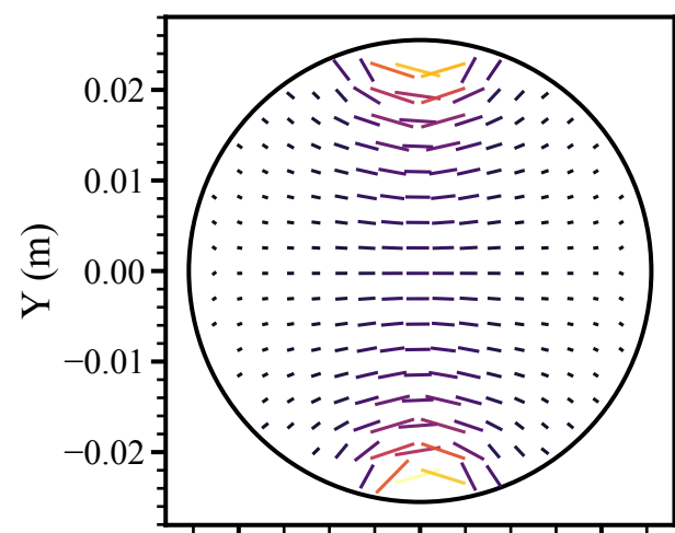
Psammitic schist (30°)
