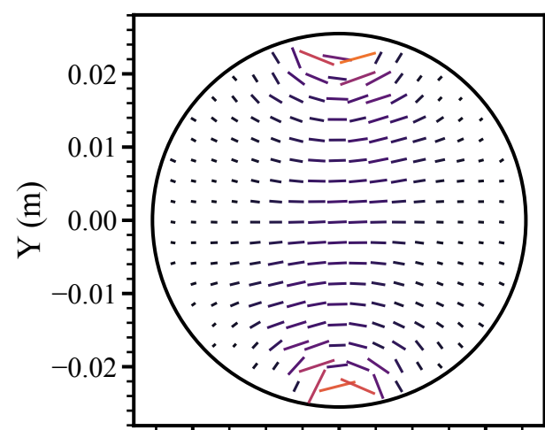
Psammitic schist (60°)
