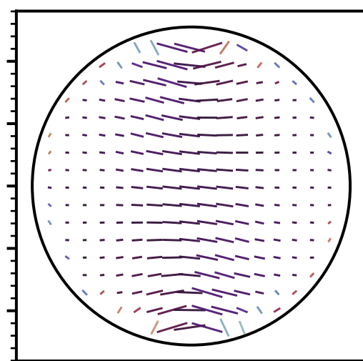
Augen gneiss (45°)
