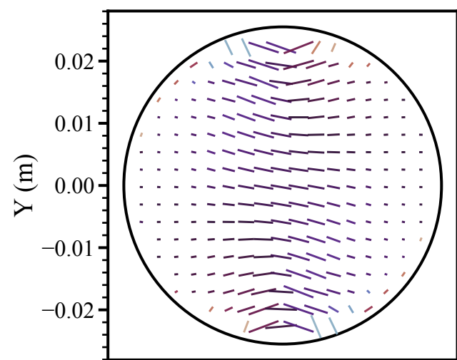
Augen gneiss (60°)
