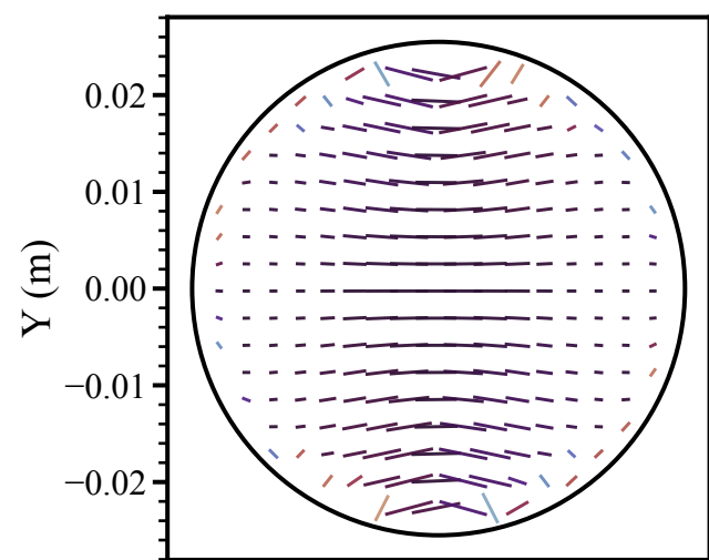
Augen gneiss (30°)
