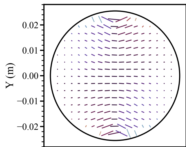
Augen gneiss (90°)
