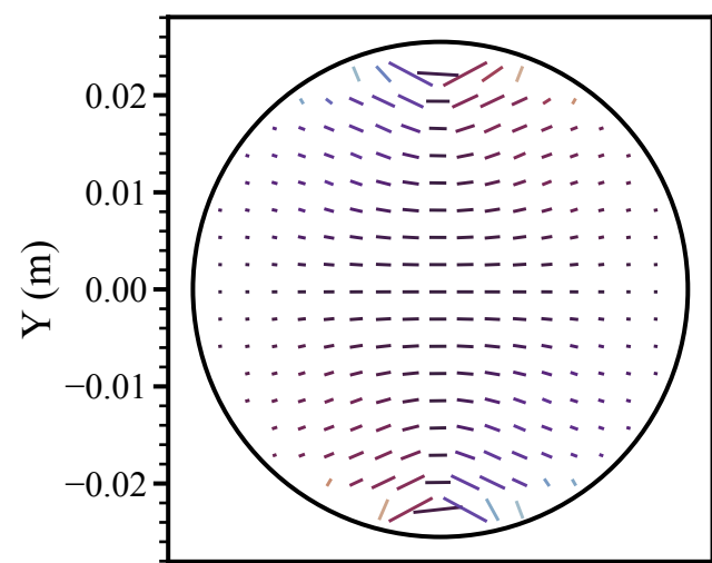
Augen gneiss (90°)
