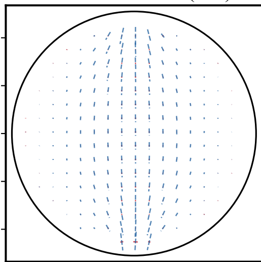
Psammitic schist (75°)
