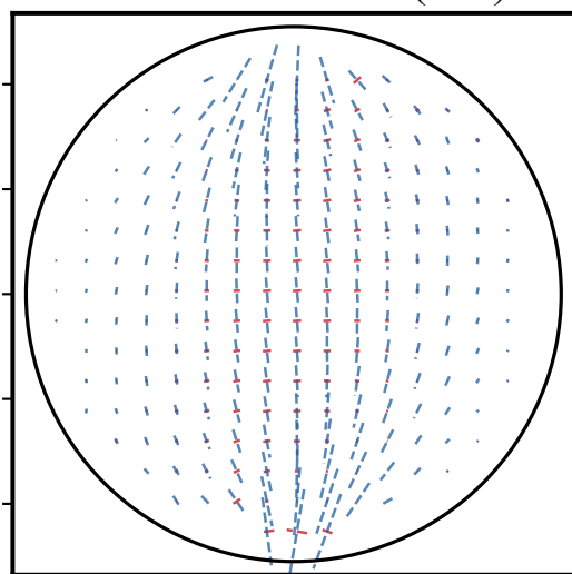
Psammitic schist (45°)
