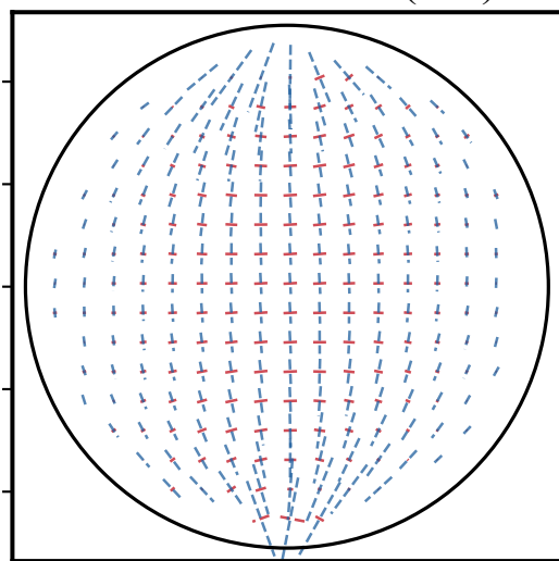
Psammitic schist (15°)
