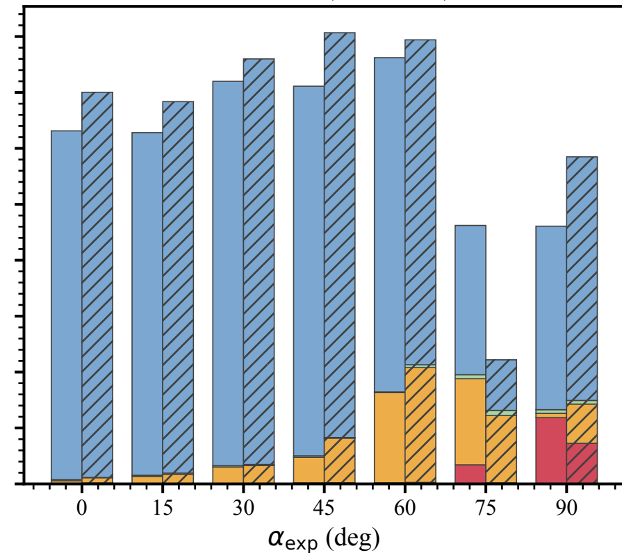
Extensional (-0.50 MPa)
