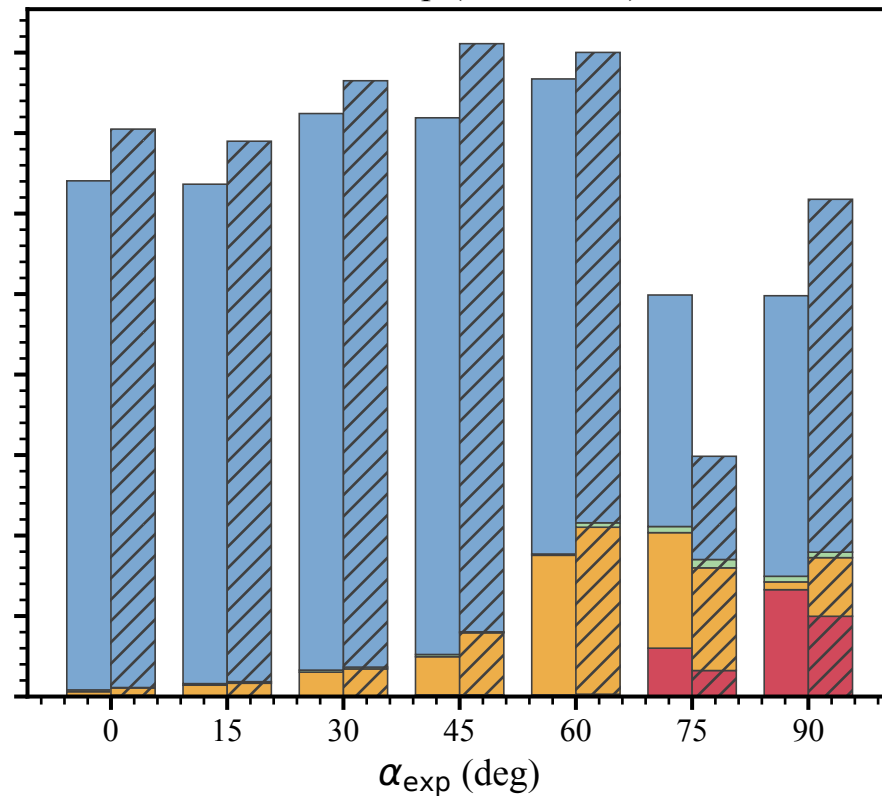
Strike-Slip (+0.00 MPa)
