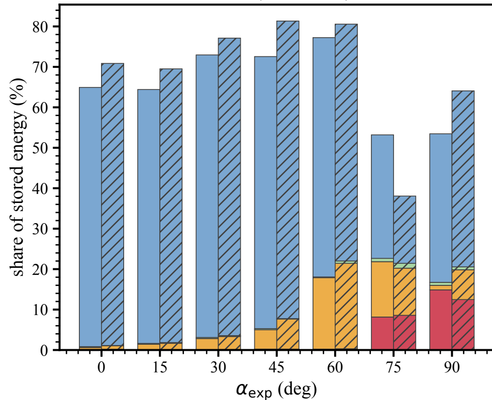
Thrust (+0.50 MPa)
