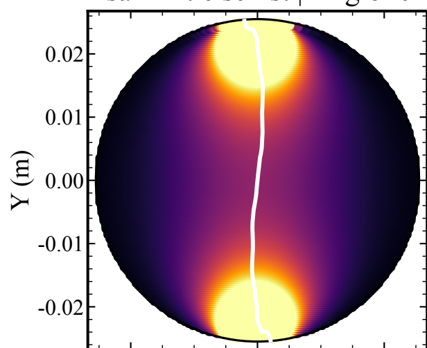
Psammitic schist | Angle=30°
