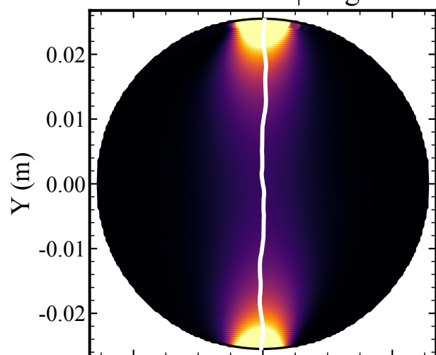
Psammitic schist | Angle=90°
