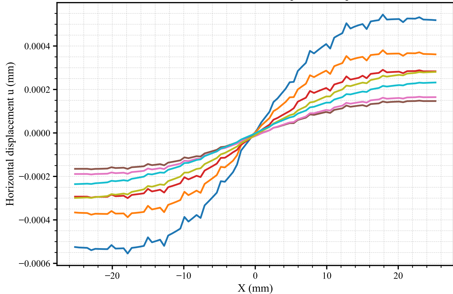
Mean mid-section horizontal displacement profiles
