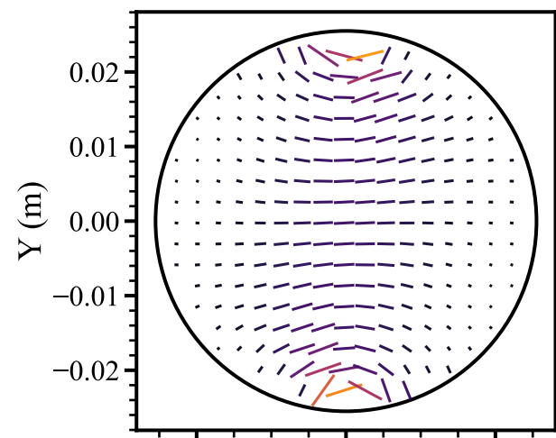
Augen gneiss (90°)
